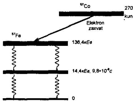
23.11-rasm. ^{57}\text{Co} \rightarrow ^{57}\text{Fe} yemirilish chizmasi.
