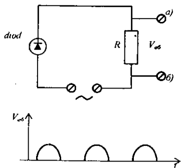
27.18-rasm. Oddiy to'g'rilagich.
