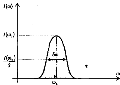
21.3-rasm. Nurlanish chizig'ining formasi.
