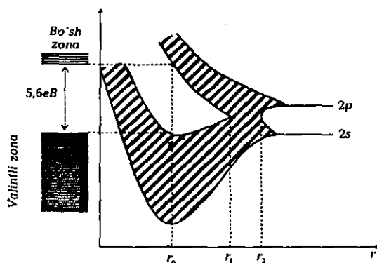
27.10-rasm. Uglerod kristalining zonalar modeli.
