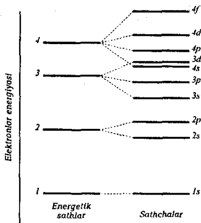
26.4-rasm. Energetik sathlar va sathchalar
