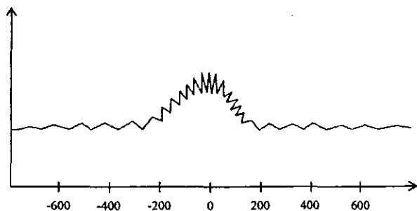
29.25-rasm. Djozefsonning ikkita tunnel o'tishi parallel ulanganda magnit maydonga bog'liq bo'lgan tokning o'zgarish grafigi.
