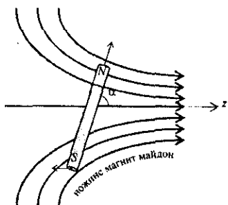
18.5-rasm. Nojins magnit maydonda magnit dipol.
