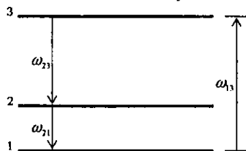
32.9-rasm. Uch sathli sistema.
