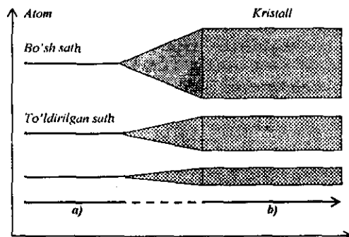
27.3-rasm. a) alohida olingan atomning energetik sathlari; b) kristalda hosil bo'lgan energetik zonalar.
