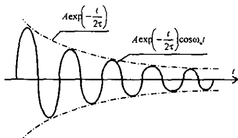
21.1-pasm. Ekspontensial so'nuvchi tebranish jarayon deyarli davriy bo'lib, tebranish chastotasi taxminan \omega_0 ga teng.
