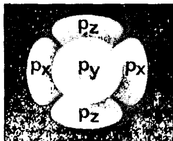
25.3-rasm. Azot atomining 3 ta 2r elektroni ( r , orbitalning 2-pallasi rasmda ko'rsatilmagan).
