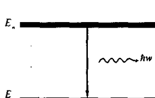
23.4-rasm. E_n dan E_m ga o'tish.
