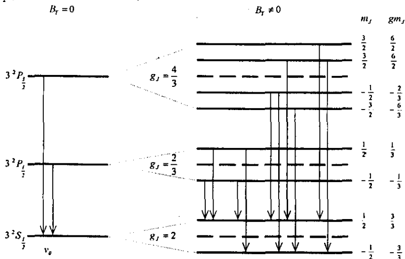
19.4-pasm. Atom sathlarining kuchsiz magnit maydonda Zeyeman anomal ajralishi
