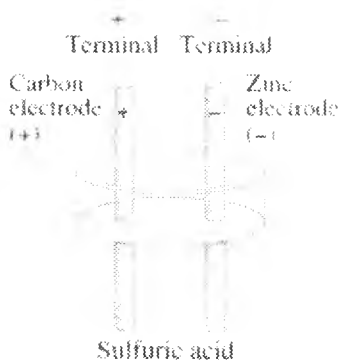
Rasm. Eng sodda galvanik element.
