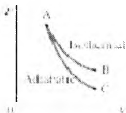
10-5- rasm. PV diagrammada ideal adiabatik (AC) gaz uchun izotermik (AB) jarayon
