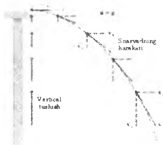
1-6-rasm. Gorizontali otilgan snaryadning harakati
