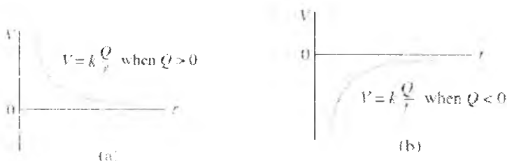
15-2-rasm. Birlik nuqtaviy zaryad Q (a) musbat, (b) manfiy bo'lganda undan r masofadagi potentsial U masofaning funksiyasidir.
