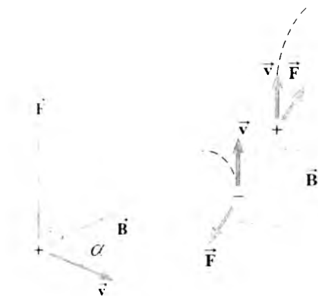
III - rasm. Harakatlanayotgan zaryadga ta'sir etuvchi Lorens kuchi
