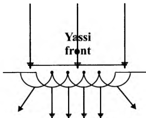
177 - rasm. Ikkilamchi to'liqlar frontining hosil bo'lishi
