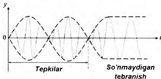
166 - rasmi. Toza majburiy garmonik tebranishning hosil bo'lishi
