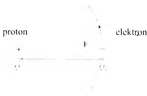
31 - rasm. Elektronning protonga ta'sir kuchi
