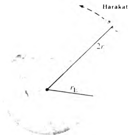
18 - rasm. Kosmik kema r = 2r_1 ga teng orbitada aylanadi
