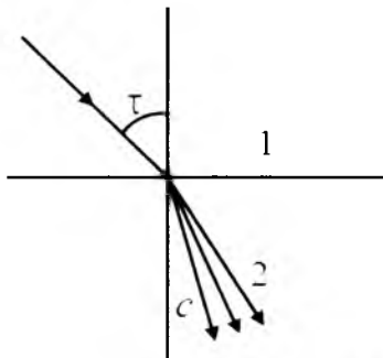
218 - rasm. Yorug'lik nuri "yelpig'ich"ining hosil bo'lishi
