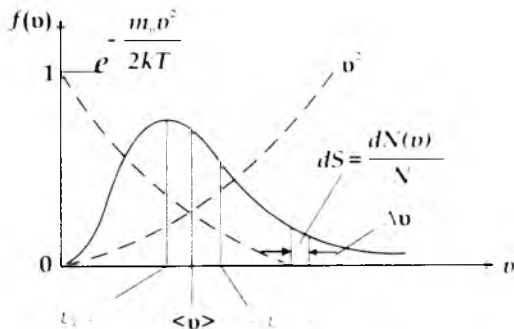
253 - rasm. Ideal gaz molekulalarining tezlik bo'yicha taqsimoti
