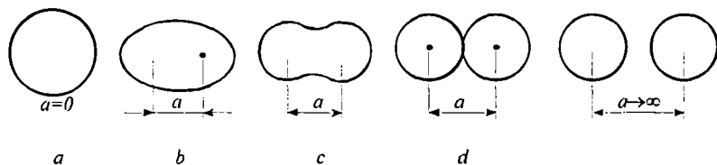
5.11-rasm. Tomchi modeliga asosan yadroning bo‘linishi.
