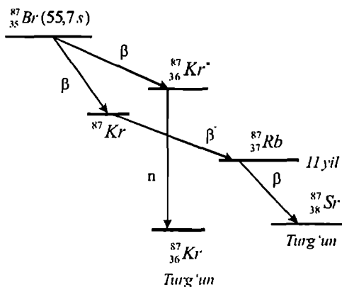
5.14-rasm. Brom-87, Kripton-87, Rubidiy-87 yadrolarining yemirilish sxemalari.
