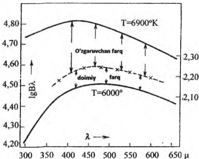
3-rasm. Rangli nurlanish haroratini aniqlash.
