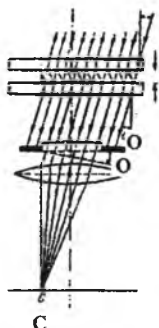
47-rasm. Fabry-Pero interferometri.
