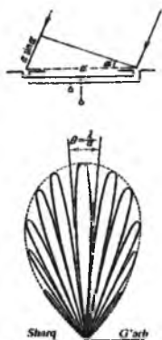
17-rasm. Sodda radiointerferometr va uning yo'nalganlik diagrammasi.
