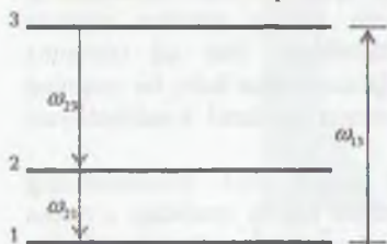
32.9-rasm. Uch sathli sistema.
