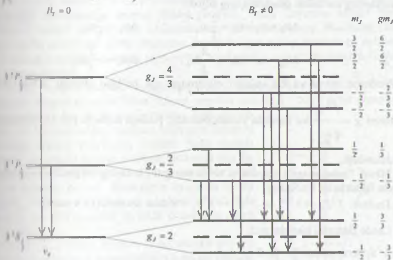
19.4-rasm. Atom sathlarining kuchsiz magnit maydonda Zeeman anomal ajralishi
