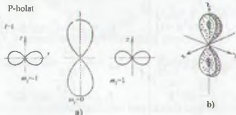
17.8-rasm. a) \theta - burchakka bog'liq bo'lgan p_\theta = |\theta_{1,0}|^2 va
