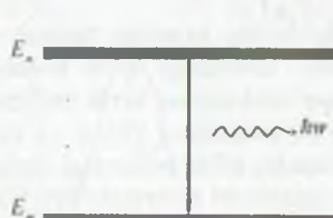
23.4-rasm. E_n dan E_m ga o'tish.
