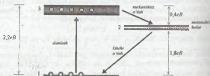
22.5-rasm. 3 sathli lazerning energetik chizmasi (yoqut misolida).
