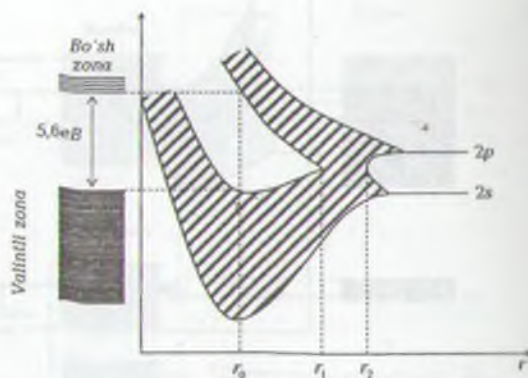
27.10-rasm. Uglerod kristalining zonalar modeli.
