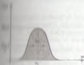
21.2-rasm. Spektral chiziqlarning Dopler broadenligi.
