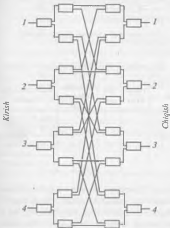
10.9-rasm. Shpenkening KSS sxemasi
