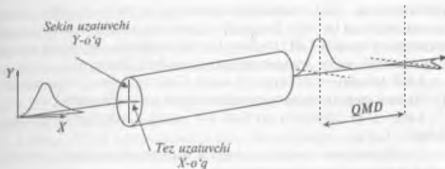
2.22-rasm. Qutblangan moda dispersiyasining hosil bo'lishi
