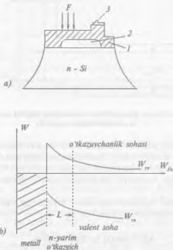
4.9-rasm. Shottki to'siqli fotodiodning tuzilishi (a) va energetik diagrammasi (b):
