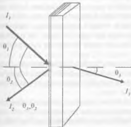
9.2-rasm. Yupqa pardali filtrning tuzilishi va ish jarayoni:
