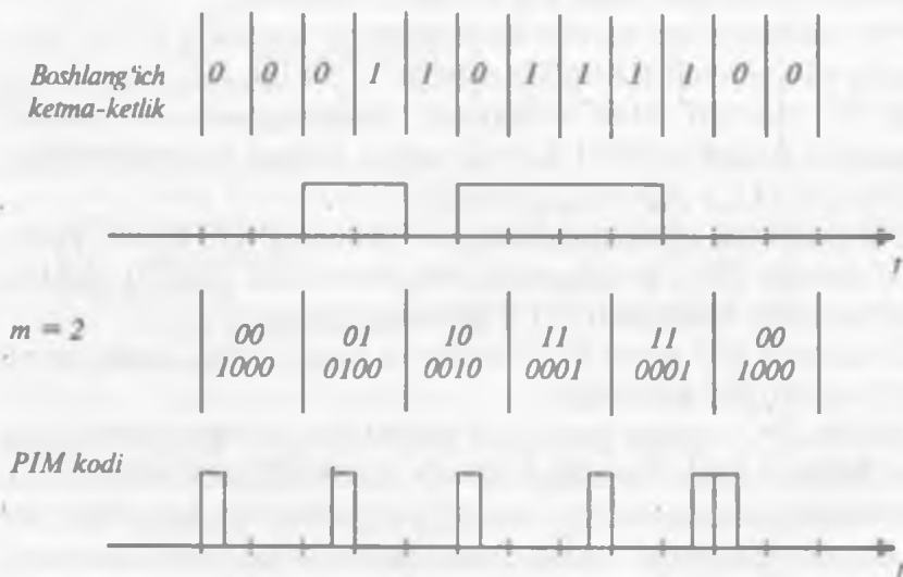
11.8-rasm. PIM kodining shakllanishi
