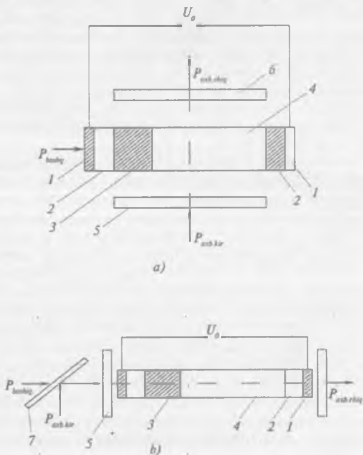
14.1-b rasm. Perpendikular turdagi (a) parallel turdagi (b) yorug'lik bilan boshqariladigan qulfnng sxemasi
