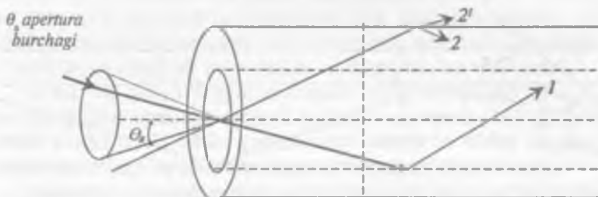
2.13-rasm. Optik tolani apertura burchagi
