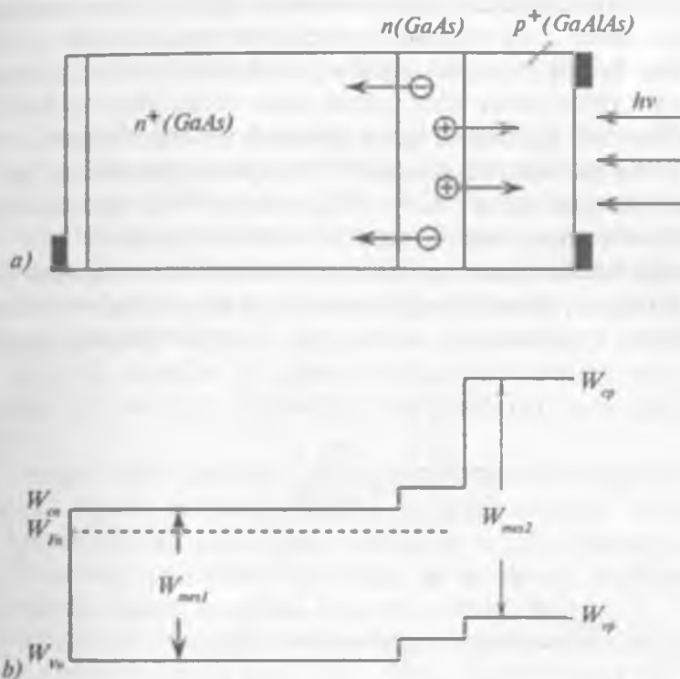
4.8-rasm. Geteroo'tishli fotodiodning tuzilishi (a) va energetik diagrammasi (b)
