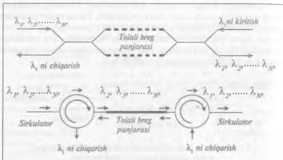
9.7-rasm. Tolali bregg panjarasidan kanallarni kiritish va chiqarish uchun foydalanish
