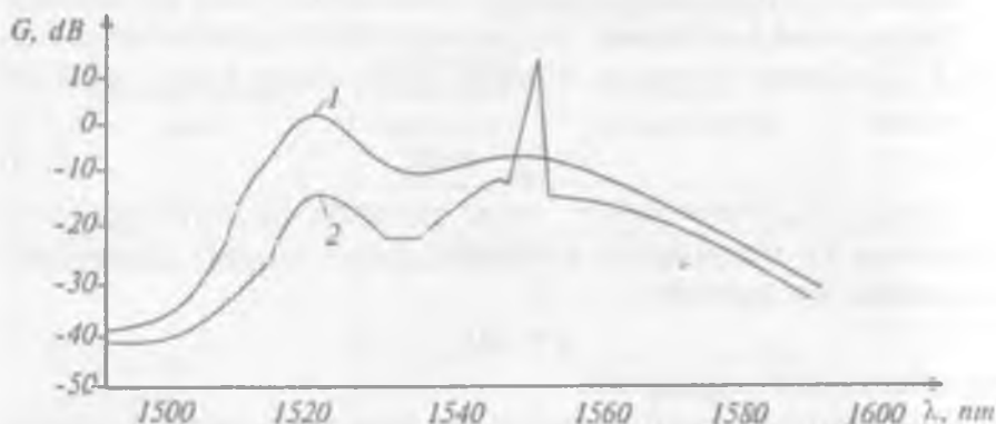
5.9-rasm. Totali optik kuchaytirgichning chiqish nurlanish spektri:
