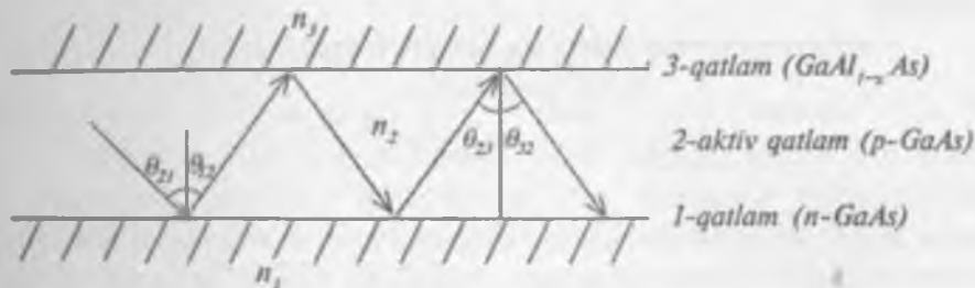
3.17-rasm. Geteroo'tishli tuzilmalarda to'lqin uzatish
