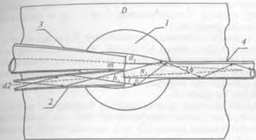
7.8-rasm. Y-tusdagi nosimmetrik tarmoqlagichning tuzilish sxemasi
