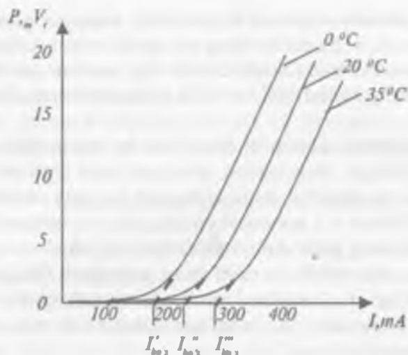
3.19-rasm. Lazer diodi vatt-ampere xarakteristikasining haroratga bog'liq ravishda o'zgarishi
