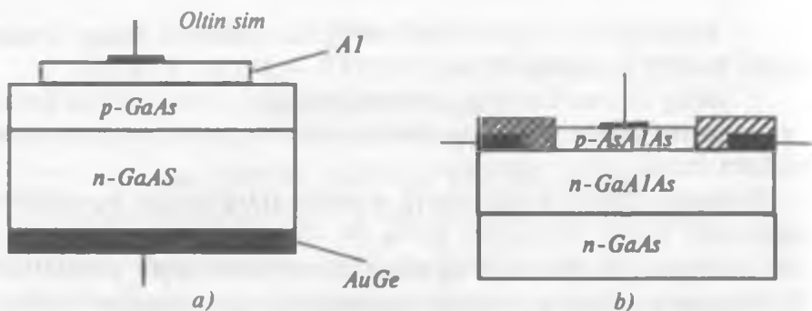
3.1-rasm. Yorug'lik diodining tuzilishi
