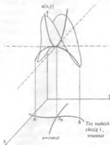
III.1-rasm: Egar nuqta
