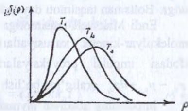
5-chizma. Temperatura qiymati-ning o'zgarishiga qarab Maksvell taqsimoti grafigasining o'zgarishi T_1 < T_2 < T_3
