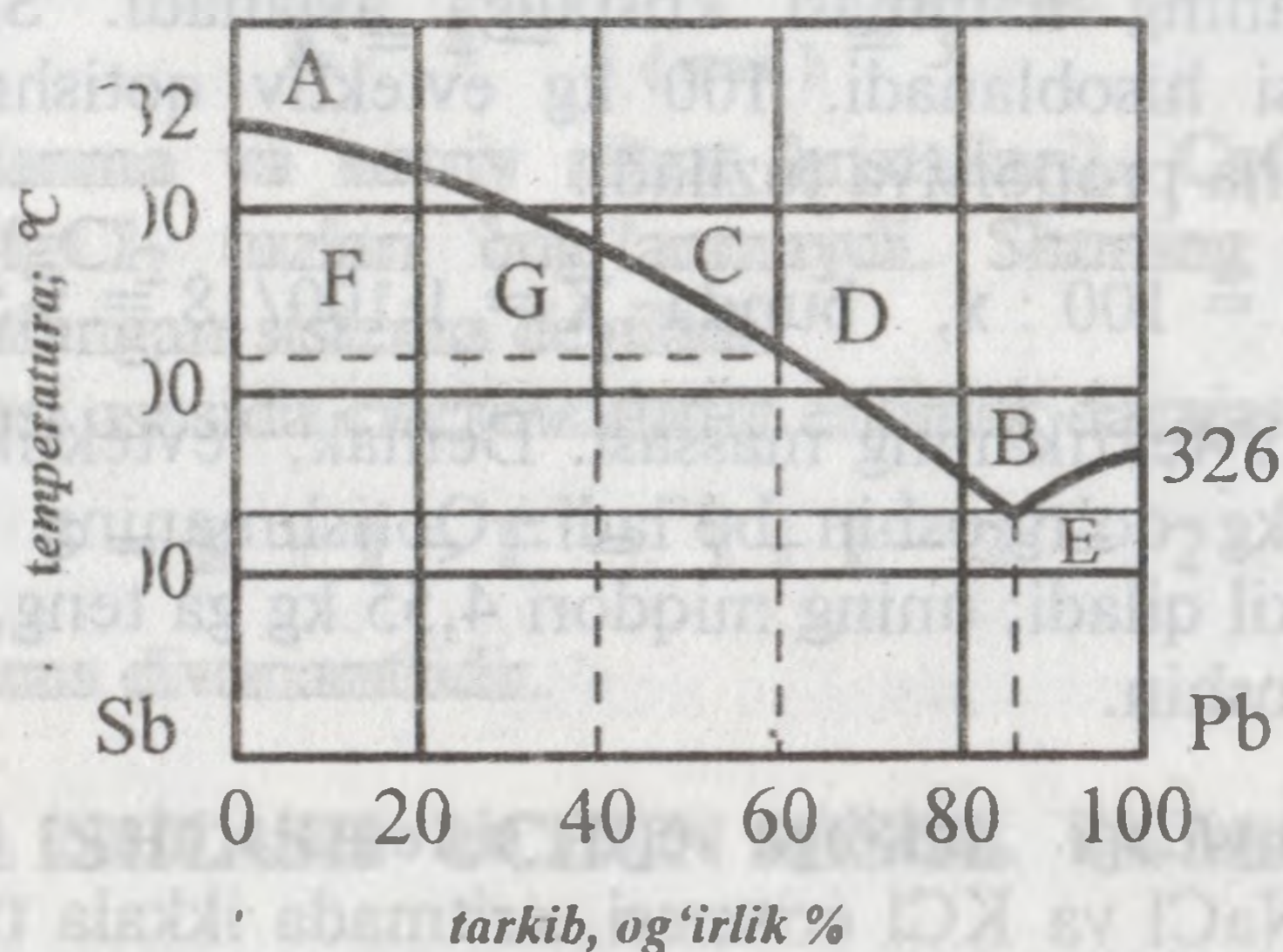
4.1-rasm. Sb – Pb sistemaning holat diagrammasi.
