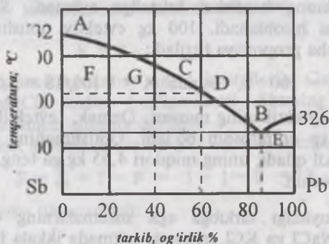
4.1-rasm. Sb – Pb sistemaning holat diagrammasi.
