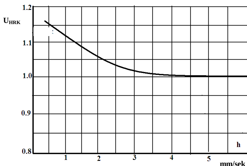
3.2- rasm. YOm g'ir intensivligining ho'l razryadlanish kuchlanishiga ta'siri.
