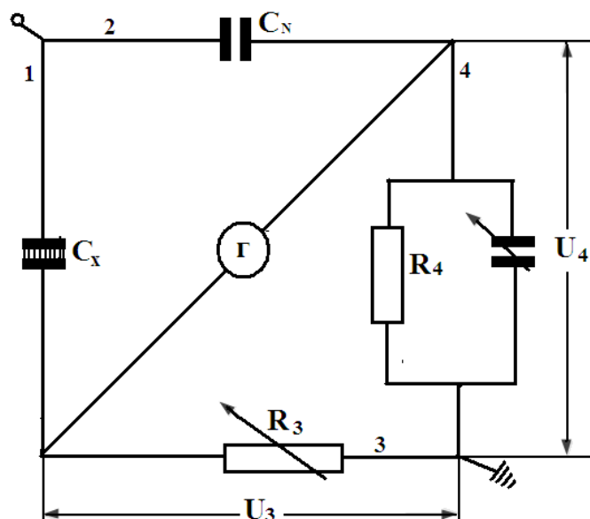
6.7- rasm. Shering ko'prigining printsipliy sxemasi
