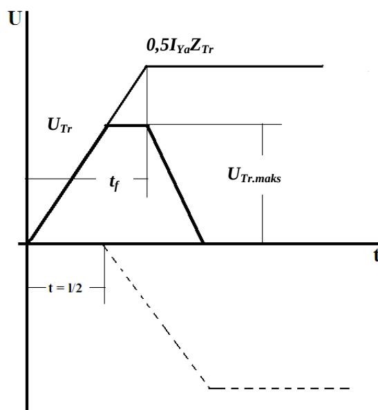
7.10- rasm. Tayanchlar oralig'ining o'rtasida trosiga yashin urilgandagi kuchlanish impuls.
