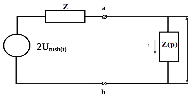
7.6- rasm. Liniyada singan to'liqinning amplitudasini aniqlash uchun foydalaniluvchi almashtirish sxemasi: Z(r) – tugunning ekvivalent qarshiligining operator ko'rinishida ifodalanishi.
