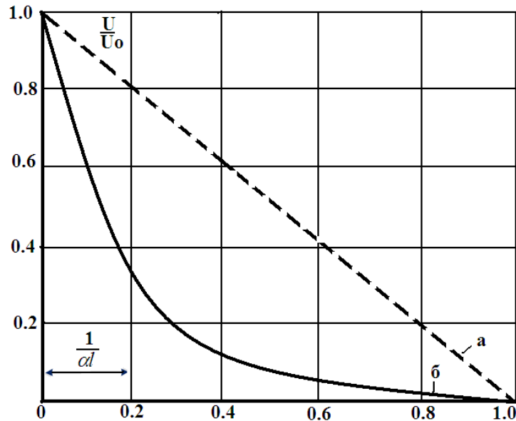
5.6- rasm. \alpha l = 5 ga teng bo'lgan chulg'am bo'ylab kuchlanishning boshlang'ich taqsimlanishi.
