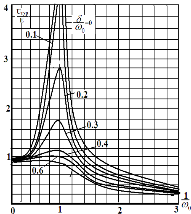
7.20- rasm. \frac{\delta}{\omega_0} ning har hil qiymatlari uchun rezonans egri chizig'i \frac{U_{ur}}{E} = f\left(\frac{1}{\omega_0}\right) ning ko'rinishi
