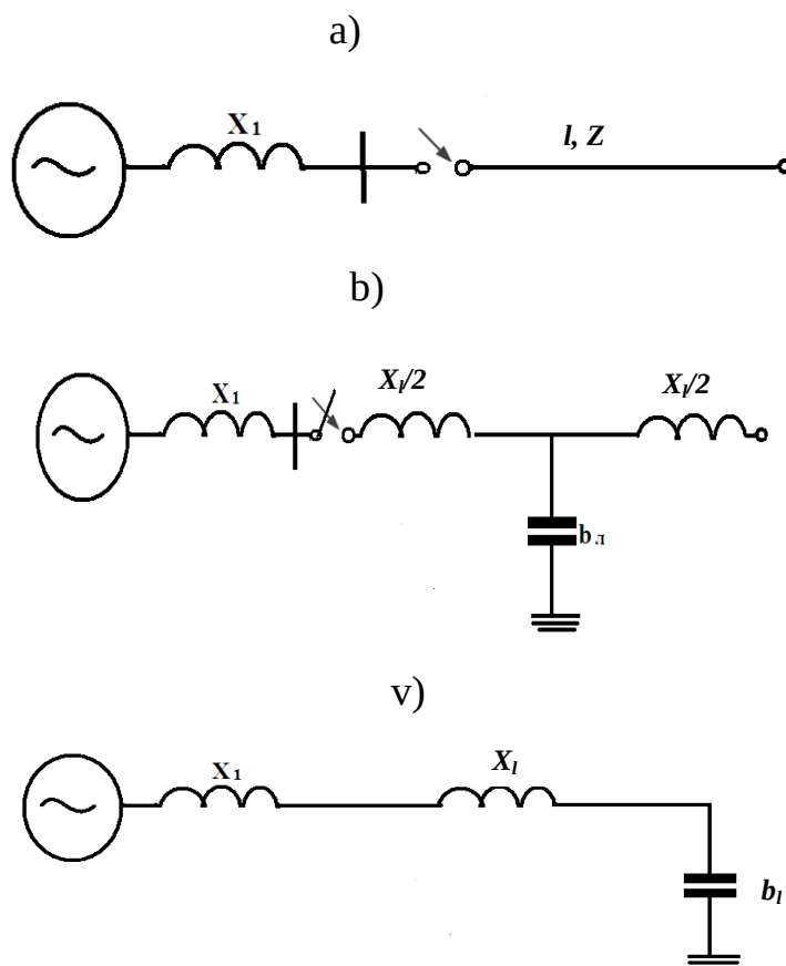
7.11- rasm. Liniyani ulashda o'takuchlanishni hisoblash uchun sxema.
