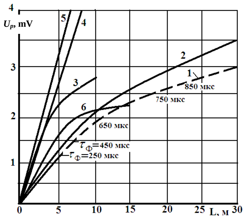
2.9- rasm. Havo oralig'ining razryadlanish kuchlanishi. Musbat qutbli kommutatsiya impulsi: 1 – “sterjen – tekislik” oralig'i uchun 50% li razryadlanish kuchlanishining eng kam qiymatida; 2 – “sterjen–tekislik” oralig'i uchun impuls frontining davom etish vaqti \tau_\Phi = 250 mks bo'lganda; 3 – “sterjen–sterjen” oralig'i uchun \tau_\Phi = 2500 - 3000 mks bo'lganda. CHaqmoqli impuls 1,2/50 mks; 4 – sterjen – tekislik musbat qutbli; 5- sterjen – tekislik manfiy qutbli; 6 – 50 Gts bilan o'zgaruvchi kuchlanish.
