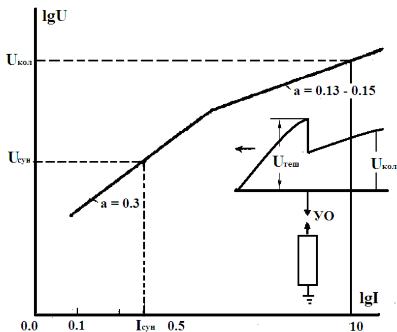
8.11- rasm. Ventilli razryadlagichning ishlash printsiipi va uning ishchi qarshiligini volt – amper xarakteristikasi (razryalagich diskining diametri d = 130 mm, I kiloamperda)
