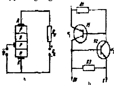
VII.16-rasm. Tiristor.
