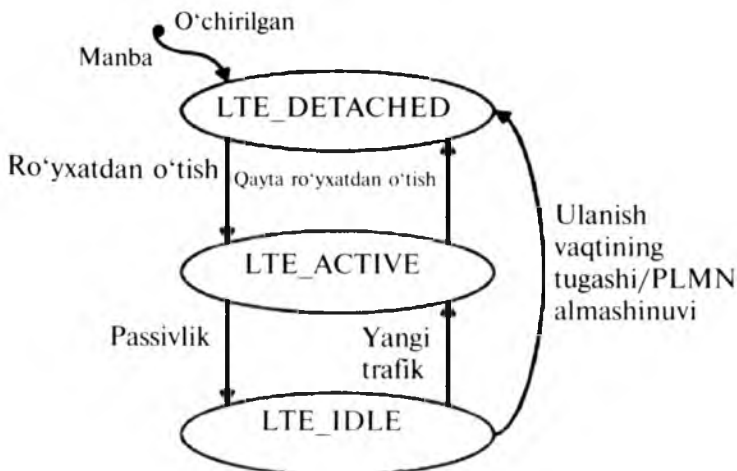
16.1-rasm. LTE tizimida AUning mobillik holatlari.
