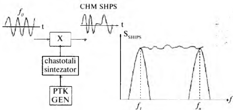
12.2-rasm. Chastotali sintizator.
