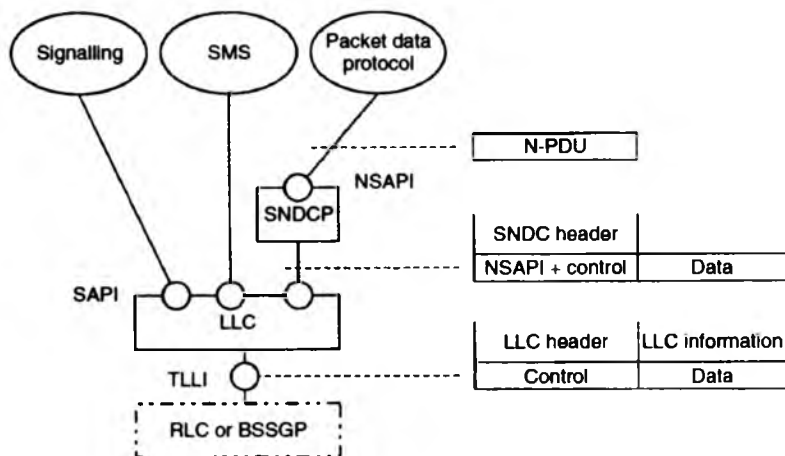
2.1-rasm. Tizimli protokollarni multipleksirlash.
