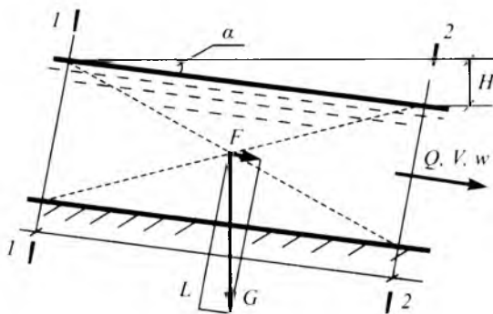
32-rasm. Suv manbasining quvvatini aniqlash.
