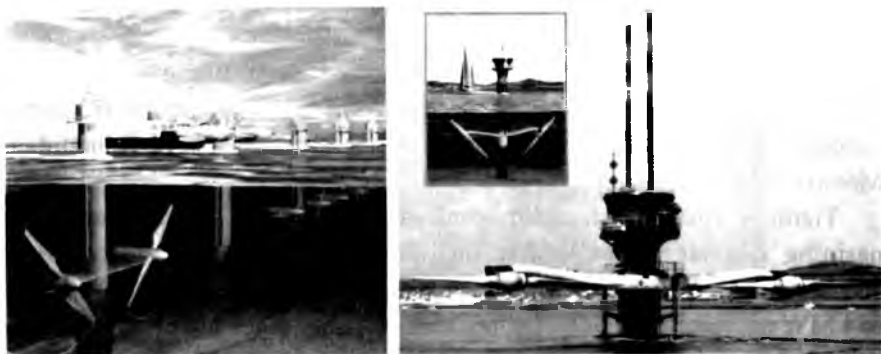
15-rasm. Suv sathining ko'tarilib-tushish prinsipi asosida ishlaydigan eng katta turbina.
