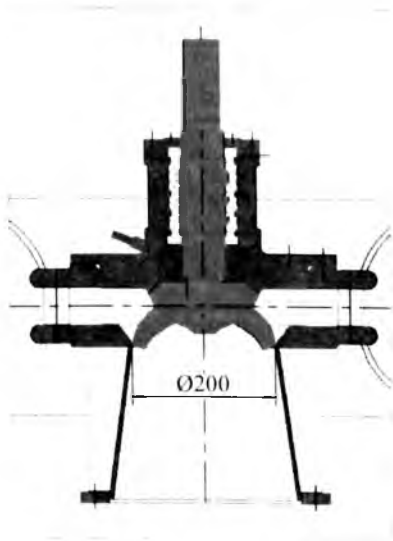
39-rasm. 20 ПпД parrakli diagonal turbinaning ishchi holatidagi ko'rinishi (a) o'rnatilish sxemasi va (b).
