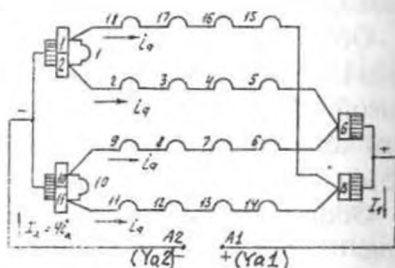
27.10-rasm. 21.9-rasmda ko'rsatilgan chulg'am parallel shohobchalari ulanishining prinsipial elektr sxemasi.
