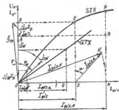
20.3-rasm. Sinx generator EYK larining amc (Potye) diagrammasi.
