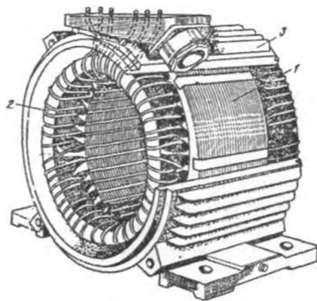
II.1-rasm. O'zgaruvchan tok mashinasining statori: 1 – stator po'lat o'zagi; 2 – stator chulg'ami va 3 – korpus (tana).
