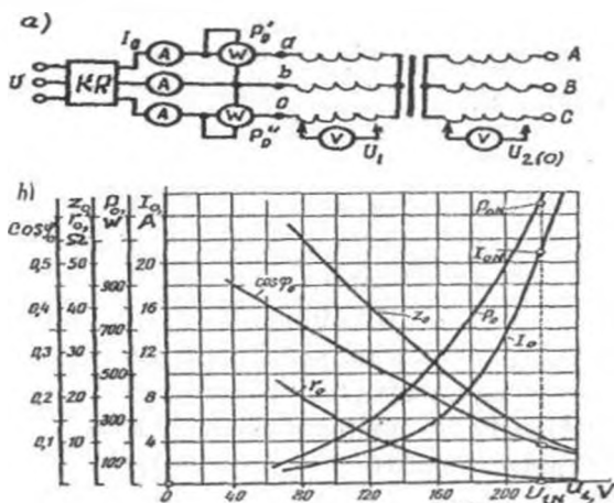
3.3-rasm. Quvvati S_N = 100 \text{ kV} \cdot \text{A} ; U_{1N} / U_{2N} = 6,3 / 0,22 \text{ kV} ; chulg'umlari Y/Y ulangan, uch fazali transformatorning salt ishlash tajribasini o'tkazish sxemasi (a) va salt ishlash xarakteristikalari (b); KR — kuchlanishni rostlagich.
