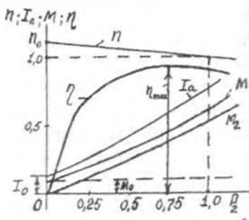
31.4-rasm. Parallel qo'zg'atishli motorning ish xarakteristikalarini
