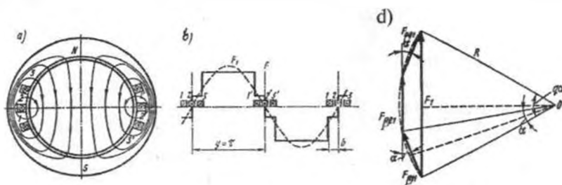
10.16-rasm. Ikki qutbli mashinaga oid ikki qatlamli taqsimlangan stator chulg'amining ko'ndalang qirgimi (a), chulg'am MYK ning taqsimlanish diagrammasi (b) va stator pazlarida taqsimlangan g'altaklar MYK larining 1-garmonika vektorlarini qo'shish diagrammasi (d)
