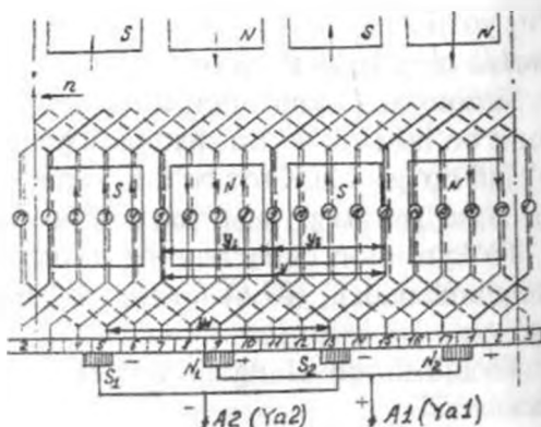
27.11- rasm. Oddiy chap yo'lli to'liqinsimon chulg'am sxemasi ( Z_1 = S = K = 17 ; 2p = 4 ; y_1 = 4 ; y = y_k = 8 ).
