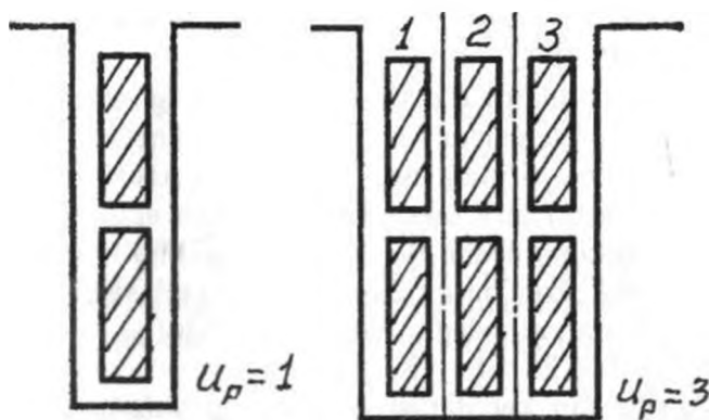
27.7-rasm. Yakorning bitta (a) va uchta (b) elementar pazdan tarkib topgan real pazlari.
