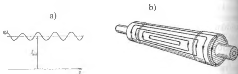
21.2-rasm. Sinxron generatorning nosimmetrik yuklamasida qo'zg'atish chulg'ami tokining o'zgarish shakli (a) va turbogenerator rotorida teskari ketma-ketlik qilgan toklar o'tadigan yo'llar sxemasi (b).
