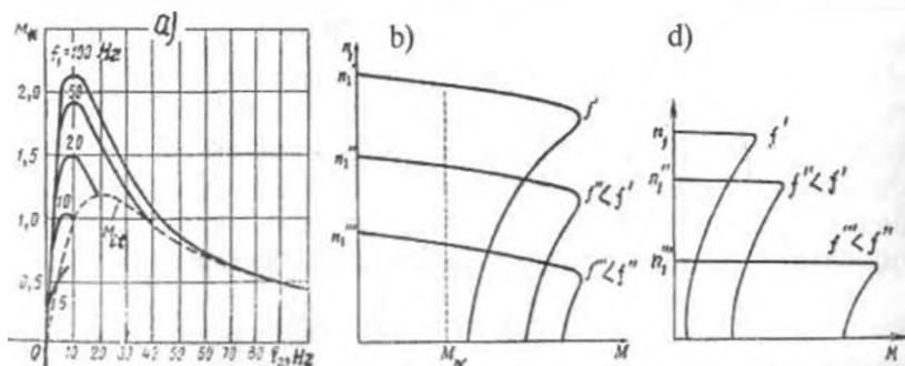
14.6-rasm. Tok chastotasi f_1 ning har xil qiymatida motor aylanish chastotasini U_1/f_1 = const sharti boyicha rostlashdagi aylantiruvchi momenti M ning chastota f_2 ga nisbatan o'zgarish grafigi (a) hamda M = const (b) va P_2 = const (d) shartlar bajarilgandagi mexanik xarakteristikalar.
