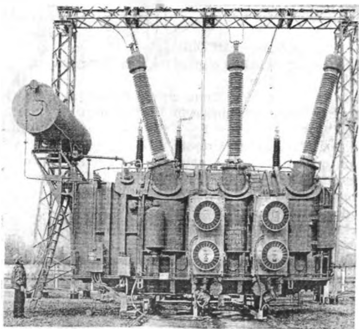
T.1-rasm. Quvvati 250000 \text{ kV} \cdot \text{A} , kuchlanishi 330 \text{ kV} , TDC-250000/330 tipli kuchlanishni oshirib beruvchi uch fazali ikki chulg'amli transformator
