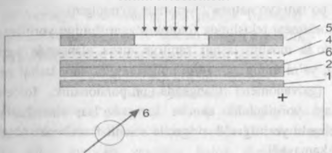
2.2-rasm. Selenli fotoelement
