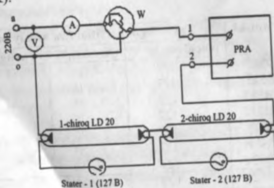
3.6-rasm. Lyuminessent chiroqlarning prinsipial ulanish sxemasi 2x20 W.
