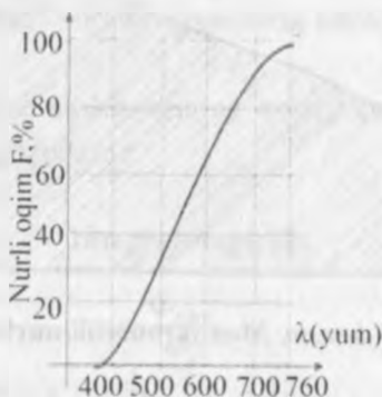
1.3-rasm. PRK-2 turidagi simobli chiroqlarning nurlanish spektri
