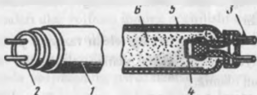
3.2-rasm. Lyuminescent chiroqlari sxemasi
