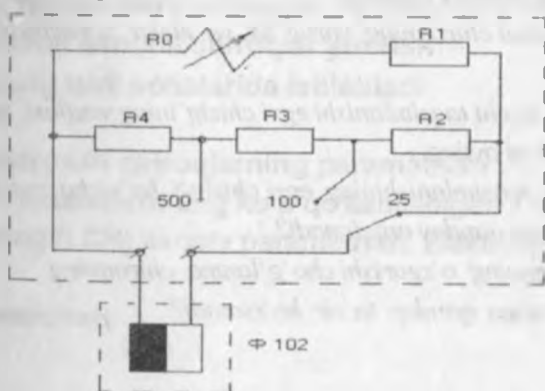
2.5-rasm. IO –16 turidagi lyuksmetrning printsipl sxemasi
