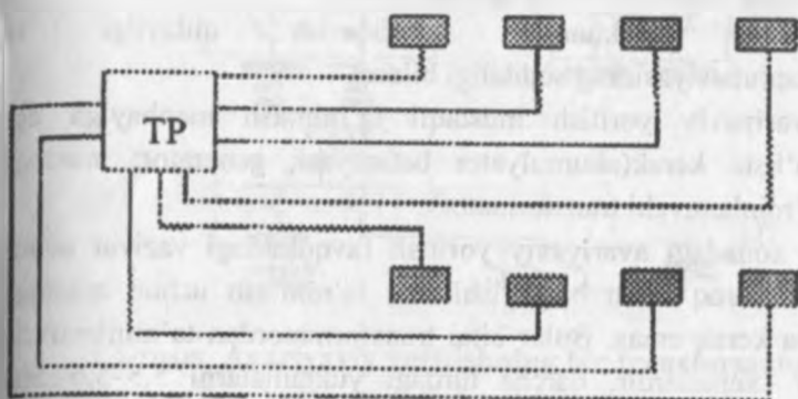
5.1-rasm. Radial (agar TQ yuklamasi 200 kVt b/sa)
