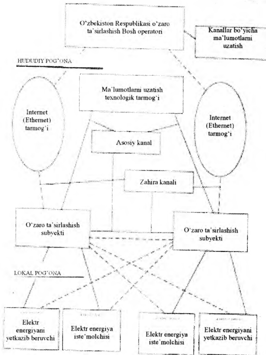
8.1-rasm. ENHAT AAO'T axborot tarmog'ining tuzilmasi
