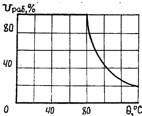
1.9-rasm. Chinnini teshuvchi kuchlanishning haroratga bog'liqligi.
