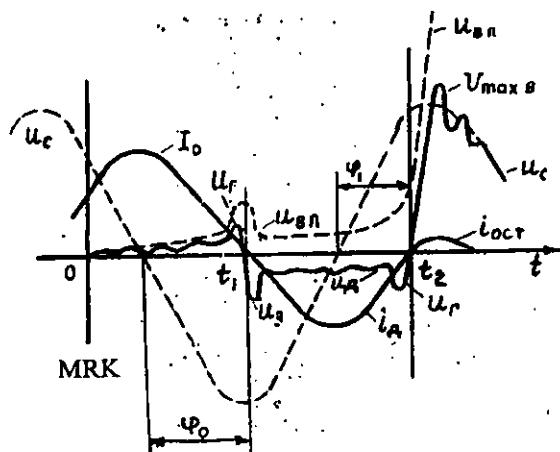
4.5-rasm. Past kuchlanishli zanjimning uzilishidagi jarayon.
