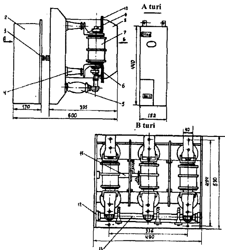
5.22-rasm. VVV- 10-2/320 turidagi uzgich.
