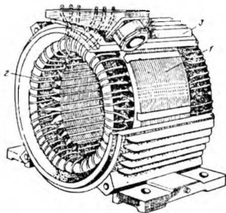
11.1-rasm. O'zgaruvchan tok mashinasining statori: 1 – stator po'lat o'zagi; 2 – stator chulg'ami va 3 – korpus (tana).
