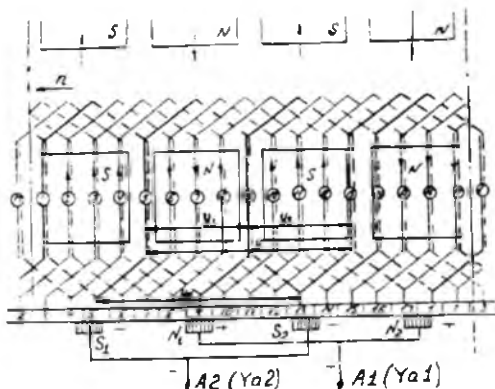
27.11- rasm. Oddiy chap yo'lli to'liqinsimon chulg'am sxemasi ( Z_p = S = K = 17 ; 2p = 4 ; y_1 = 4 ; y = y_k = 8 ).
