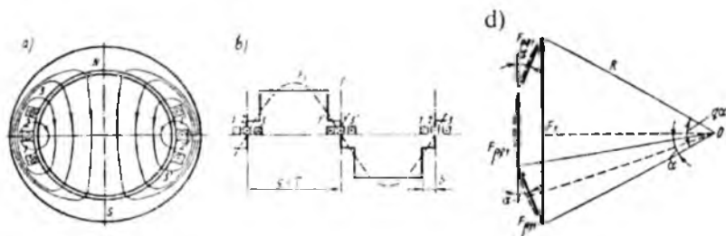
10.16-rasm. Ikki qutbli mashinaga oid ikki qatlamli taqsimlangan stator chulg'aminin ko'ndalang qirgimi (a), chulg'am MYK ning taqsimlanish diagrammasi (b) va stator pazlarida taqsimlangan g'altaklar MYK larining 1-garmonika vektorlarini qo'shish diagrammasi (d)
