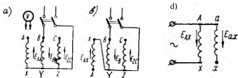
2.8-rasm. Transformatorning YK chulg'ami uchlari to'g'ri (a) va noto'g'ri (b) belgilangan uchlar uchun hamda chulg'am uchlari belgilanishini tajribada tekshirish uchun (d) sxemalar.
