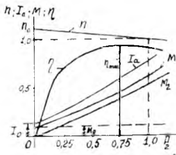
31.4-rasm. Parallel qo'zg'atishli motorning ish xarakteristikalari
