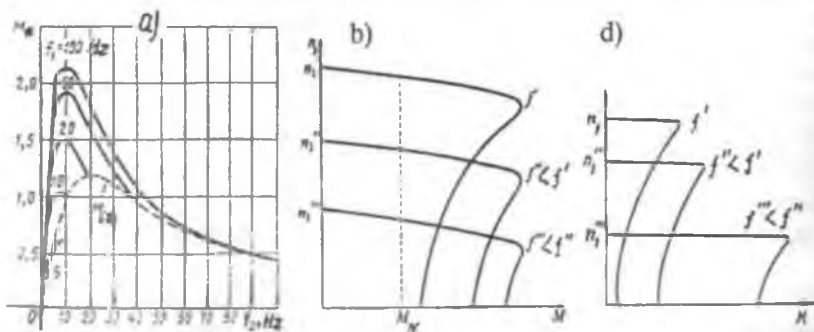
14.6-rasm. Tok chastotasi f_1 ning har xil qiymatida motor aylanish chastotasini U_1/f_1 = \text{const} sharti boyicha rostdlashdagi aylantiruvchi momenti M ning chastota f_2 ga nisbatan o'zgarish grafigi (a) hamda M = \text{const} (b) va P_2 = \text{const} (d) shartlar bajarilgandagi mexanik xarakteristikalar.
