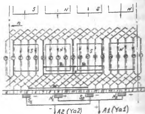
27.11- rasm. Oddiy chap yo'lli to'liqinsimon chulg'am sxemasi ( Z = S = K = 17 ; 2p = 4 ; y_1 = 4 ; y = y_k = 8 ).
