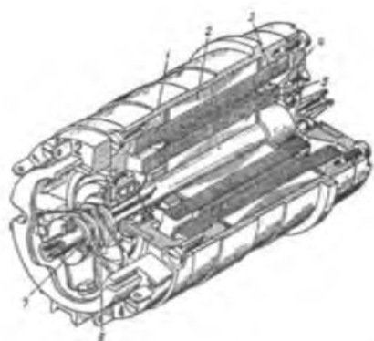
17.3-rasm. Aylanuvchi transformatorning umumiy ko'rinishi ( a ): 1 – korpus (tana), 2 – stator, 3 – stator chulg'ami, 4 – rotor, 5 – rotor chulg'ami, 6 – kontakt halqalar, 7 – cho't'kalar; b – prinsipial sxemasi.
