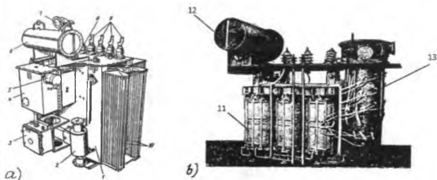
5.5-rasm. Kuchlanishi RPN usulida rostlanadigan kuch transformatorlari:
