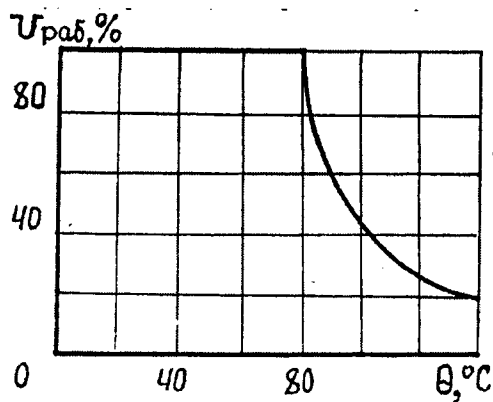
1.9-rasm. Chinnini teshuvchi kuchlanishning haroratga bog'liqligi.
