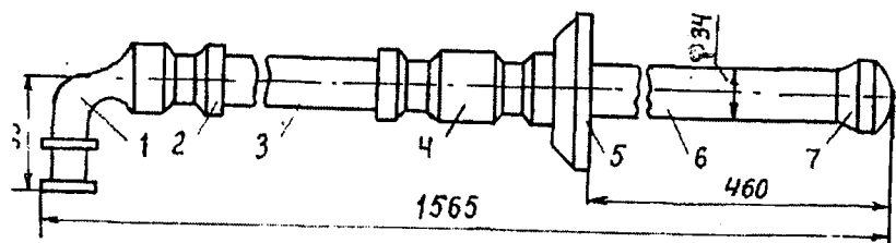
7.4-rasm. ShR — 10 turidagi 10 kB li tezkor shtanga.
