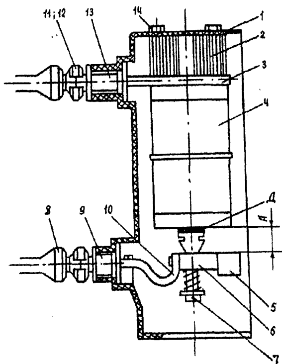
5.21-rasm. VVE- 10 turdagi uzgich qutbi:
