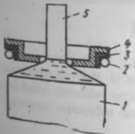
II.48-rasm. Muayyan shaklli kristallarni taglikdan o'tirish:
