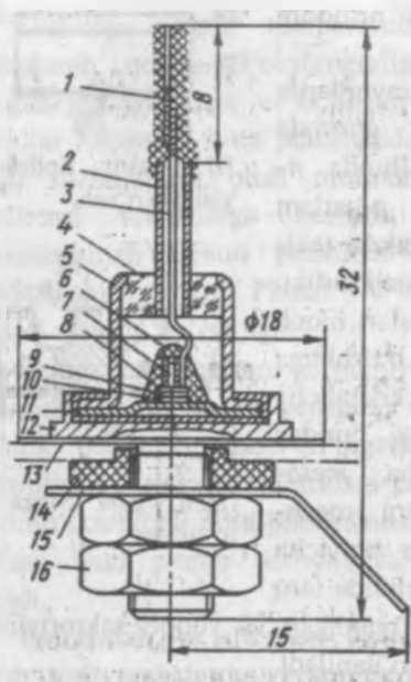
III 63-rasm Kremniy yassi diodining tuzilishi chizmasi:
