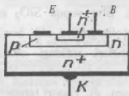
III.72-rasm. Epitaksial-planar tranzistor tuzilishi
