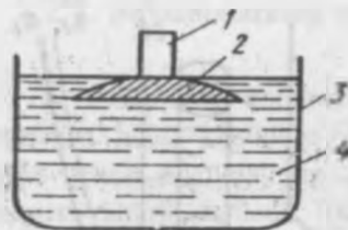
11.36-rasm. Kiropulos usulida kristallar o'stirish.
