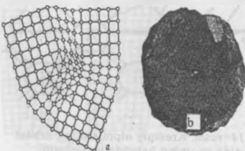
I.15-rasm. Yarimo'tkazgichlarning mozaik tuzilishi: a – mozaik tuzilish chizmasi; b – InP kristalli kesimida mozaik tuzilish.
