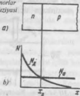
III.57-rasm. Diffuzion p - n o'tishning hosil bo'lishi
