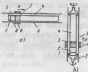
11.37-rasm. Zonaviy suyultirish usulida kristall o'stirish:
