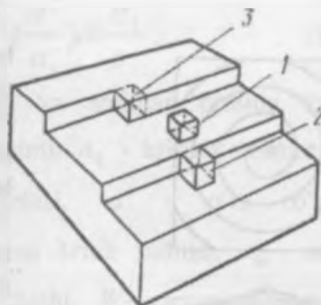
II.13-rasm. Atom - sillik sirtning o'sish modeli.
