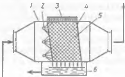
5.8-rasm. Nasdkali skrubber:
