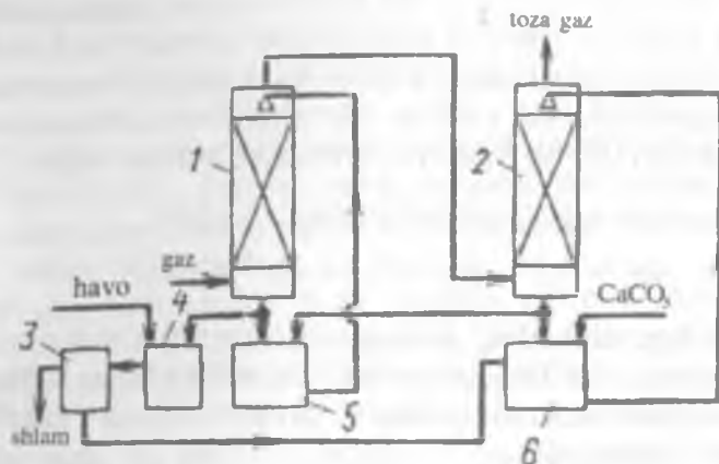
9.4-rasm. Ikki bosqichli \text{SO}_2 gazini tozalash absorbsion qurilmasi: 1,2-absorber; 3-sentrifuga; 4,5,6-yig'ichlar.
