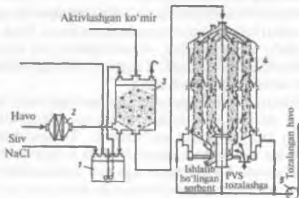
15.1-rasm. Ventilatsion tashlamalarni demerkurizatsiyalash absorbsion qurilmasining sxemasi:
