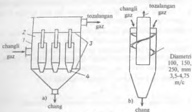
5.5-rasm. Batareyali siklon:
