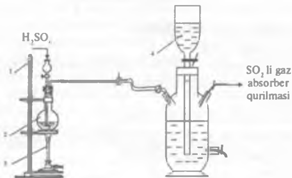
1-rasm. SO 2 gazini olish laboratoriya qurilmasi:
