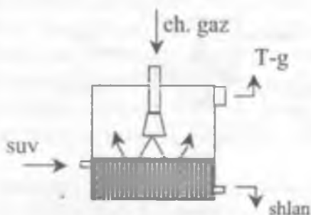
5.11-rasm. Inersion uriluvchi changyutgich.
