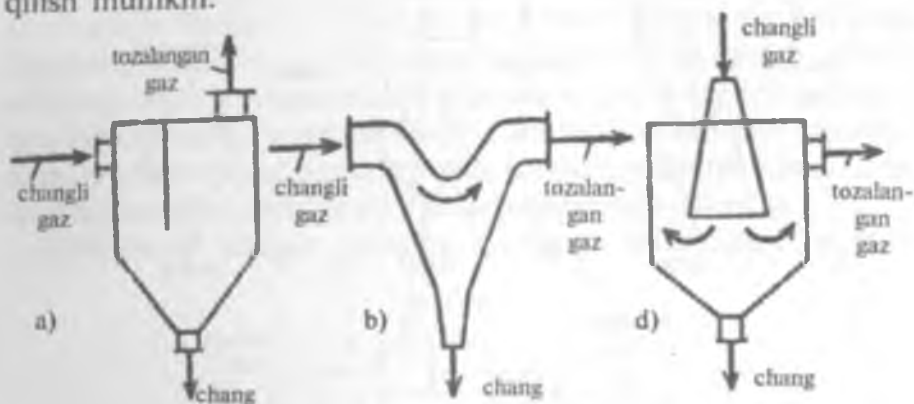
5.2-rasm. Inersion chang ushlagichlar:
