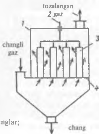
5.6-rasm. Yengsimon filtr:
