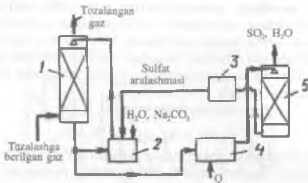
9.7- rasm. Sulfit-bisulfit usulida \text{SO}_2 gazini absorbsion tozalash: 1-absorber; 2,3- sig'imlar; 4-regenerator; 5-bug'latish (desorber) kolonnasi.
