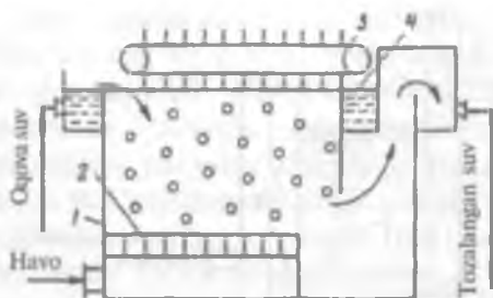
18.9-rasm. Filtrovchi plastinali flotator: 1-kamera; 2-filtrli plastinalar; 3-yig'gich; 4-shlam yig'gich.
