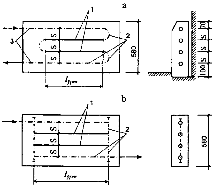
11.2-rasm. Egilib va ustunchali qilib yasalgan isitish panellarining sxemasi
