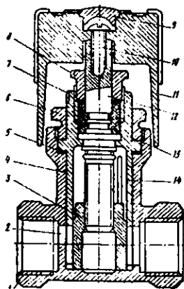
5.11-rasm. Ikki tomonlama boshqaruvchi jo'mrak – IBJ: 1 – korpus; 2 – boshqaruvchi tuynuk; 3 – shiber; 4 – buruvchi vtulka; 5 – prokladka; 6 – mahkamlovchi gayka; 7 – vtulka riskasi; 8 – salnik gaykasi; 9 – qopqog; 10 – vint; 11 – dasta; 12 – rezbali shpindel; 13 – sanlikli jipslagich; 14 – vtulkadagi paz
