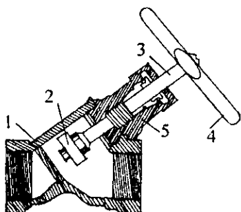
5.13-rasm. Qiyshiq shpindellik jo'mrak – QShJ
