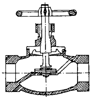
5.14-rasm. To'g'ri shpindelli jo'mrak – TShJ
