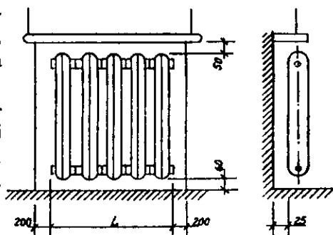
4.17-rasm. Radiatorlarning mehroblarga o'rnatilishi
