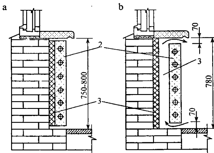
11.3-rasm. Panelli nurlanuvchi isitish asboblarning deraza tagiga o'rnatilishi
