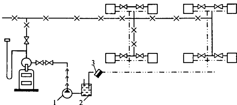
1.10-rasm. Past bosimli bug'li ochiq isitish tizimining prinsipial sxemasi
