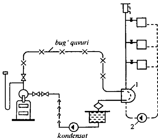
1.11-rasm. Bug'-suvli isitish tizimining prinsipial sxemasi
