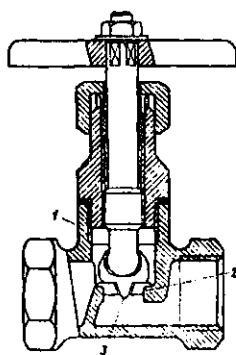
5.12-rasm. Drosselli boshqaruvchi jo'mrak – DBJ: 1 – korpus;
