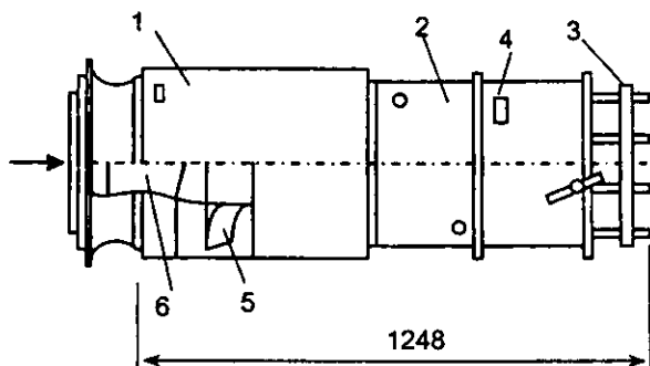
10.3-rasm. Osma isitish agregati: 1 – asbob sirti; 2 – havo isitgich; 3 – panjara klapan; 4 – ilgak (kranshteyn); 5 – parrak; 6 – elektrdvigatel
