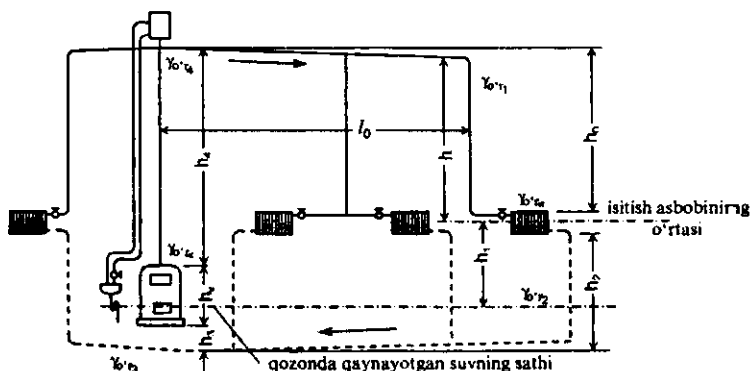
7.8-rasm. Turar joy binolarini isitish tizimi
