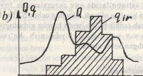
3.7. (b)-rasm. Oqimni murakkab rostdlash gidrografi
