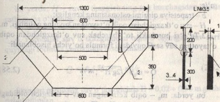
2.33-rasm. Trapetsiya shaklidagi Chipoletti (VCh-50) suv o'lchagichi: (vodoslivi), tubining kengligi 500 mm (50 sm, 1 sm-10 mm)
