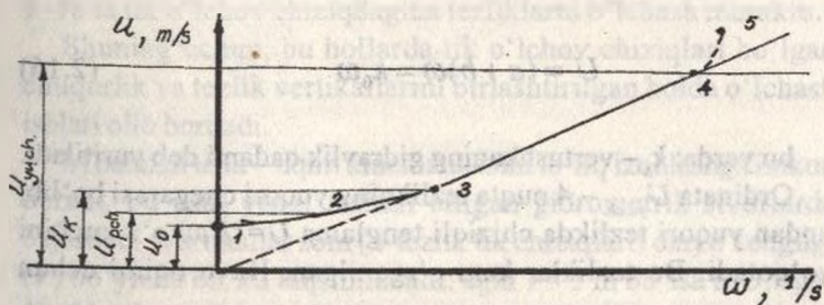
2.17-rasm. Vertushkaning darajalanish (graduировка) grafigi
