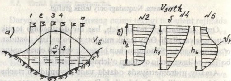
2.11-rasm. Ochiq havzada tezliklarning taqsimlanishi
