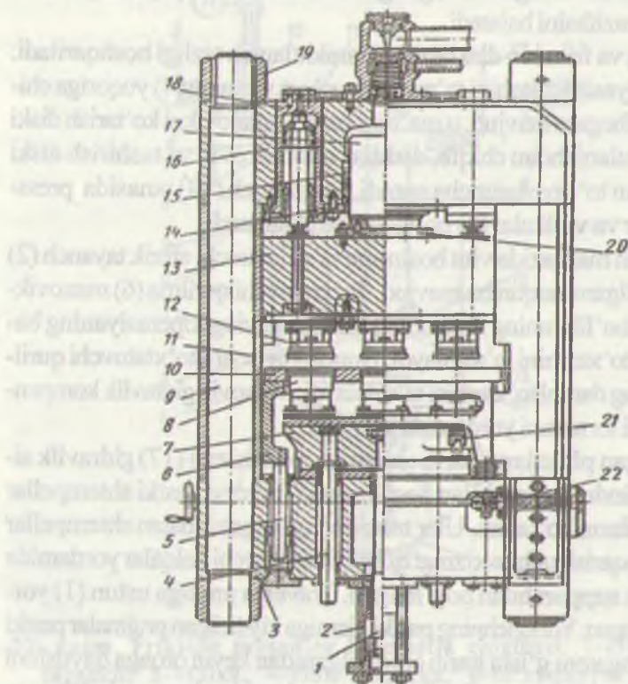
38-rasm. Gidravlik press: 1- shtok, 2,18,24 - gidrosilindr, 3 - harakatlanmaydigan plita, 4,5 - yo'llantiruvchi, 6 - ishchi stol, 7,25 - kartka, 8 - chiqaruvchi, 9 - kolonka, 10 - matrisa, 11,15 - vtulka, 12 - yuqori shtamp, 13 - harakatchan plita, 14,20 - flanes, 16 - traversa; 17 - plunjer, 19 - gayka, 21- tayanch, 22 - vintli moslama, 23 - kronshteyn, 26 - quyi roliklar, 27 - bunker.
