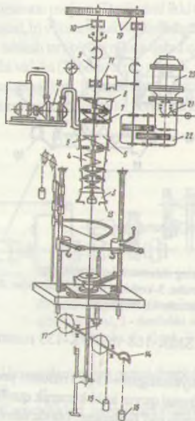
30-rasm. Tik shnekli vakuumpress: 1-qabul qiluvchi stol, 2-qabul qiluvchi stol, 3-boshcha, 4-press tanasi, 5-parrak, 6-vakuumpress, 7-g'alvirsimon panjara, 8-yuklash kamerasi, 9-tik o'q, 10, 11-podshipniklar, 12-qoplama, 13-mundstuk, 14, 15, 16, 17-bosimga qarshi sistemalar, 18-reduktor, 19-tishli uzatma, 20-elektr yuritgich, 21-friksion mufta, 22-reduktor.
