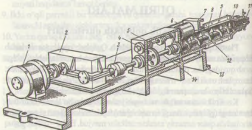
22-rasm. Lentasimon press: 1-elektryuritgich, 2-reduktor, 3-uzatkich, 4-tishli mufta, 5-tishli g'ildiraklar, 6-oraliq o'q, 7-qabul qiluvchi quti, 8-qoplama, 9-tana, 10-boshcha, 11-mundshtuk, 12-parraklar, 13-plita, 14-o'q.
