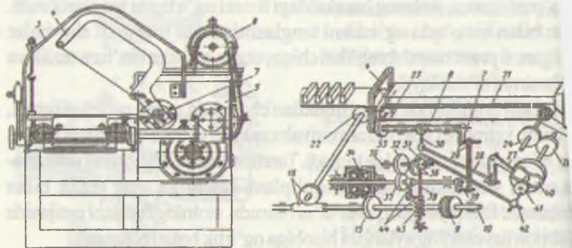
31- rasm. Qirqish stanogi: 1-qabul qiluvchi stol, 2, 21-transportyor, 3-qoplar, 4-keskich, 5-quti, 6-gilza, 7, 14, 25, 35-o'q, 8-elektryuritgich, 9-tasmali uzatma, 10-harakatlantiruvchi o'q, 11-stanina, 12-asos, 13-tishli g'ildirak, 15, 24, 26, 32, 33, 37-shesternya, 16-uzatma, 17-salazka, 18-kontr yuk, 19-valch, 20, 23-baraban, 22-rolik, 27, 44-yelka, 28, 38, 42-tyaga, 29, 39-krivoship-shatunli mexanizm, 30-provodok, 31-qayta ulagich, 34-friksion mufta, 36-ikki tomonlama kulachok, 40-kopir, 41-shayba, 43-prujina.
