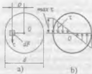
54-rasm. Buralishda urinma kuchlanishi taqsimoti; a) \sigma va \tau ortogonaligi; b) urinma kuchlanishlar epyurasi
