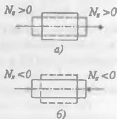
35-rasm. a) cho'zilish; b) siqilish.
