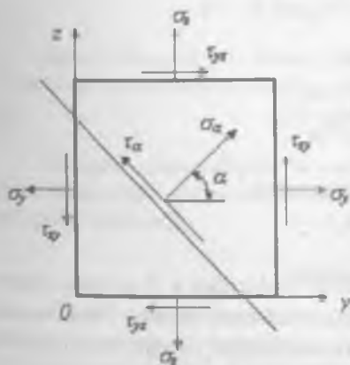
18-rasm. Boshlang'ich yassi kuchlangan holat.
