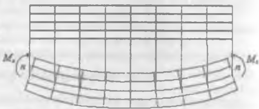
42-rasm. Sof egilish modeli.
