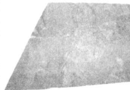
45-rasm. Brekchiya.
