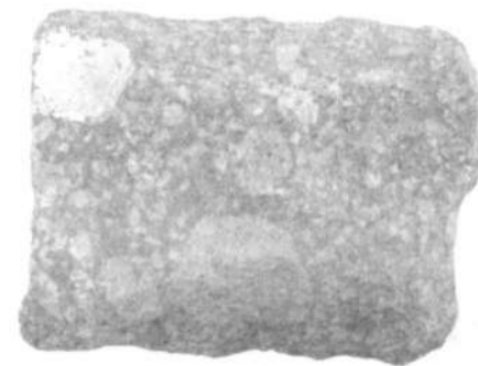
37- rasm. Traxit.
