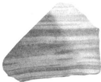
24- rasm. Serpentin.
