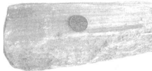
17- rasm. Gips.
