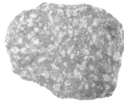
35- rasm. Andezit.
