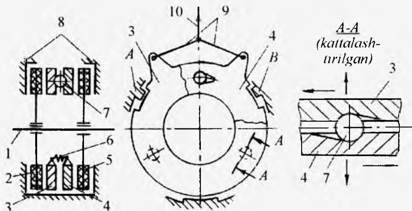
90-rasm. Servokuchaytirgichli, yopiq diskli tormoz.
