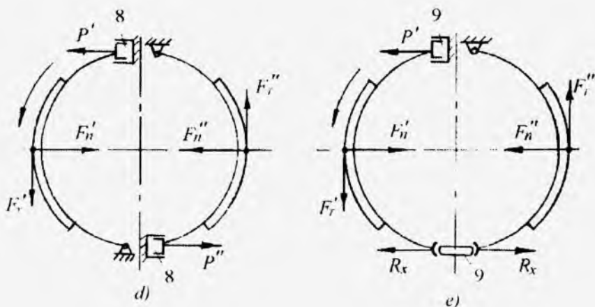
88-rasm. Barabanli tormozlar.
