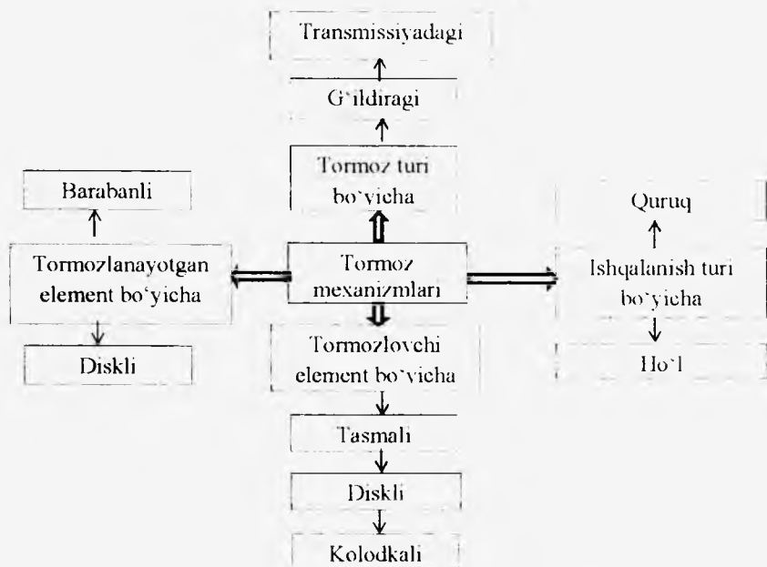
86-rasm. Tormoz mexanizmining xillari.
