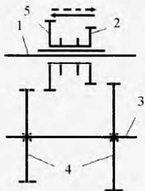
24-rasm. Shesternyalar ilashishining sodda konstruksiyasi. 1-birlamchi o'q, 2,5-siljivchi kareta shesternyalari; 3-ikkilamchi o'q; 4-shesternyalar.
