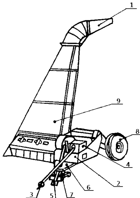
11.2-rasm. Rotorli o'to'rgich-maydalagichning sxemasi: 1-to'sqich; 2-rama; 3-kardanli val; 4-reduktor; 5-yakka shoti; 6-tirkama; 7-tayanch; 8-g'ildirak; 9-yuklagich
