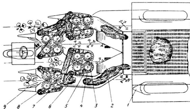
14.2-rasm. Mashinaning texnologik ish jarayoni sxemasi: 1-ketingi g'ildiraklar suyrisi; 2-ventilyator; 3-shpindellar yuritmasi; 4-shpindellarni teskari aylantirish kolodkasi; 5-shpindelli baraban; 6-havo trubasi; 7-ajratgich; 8-qabul kamera; 9-tup ko'targich
