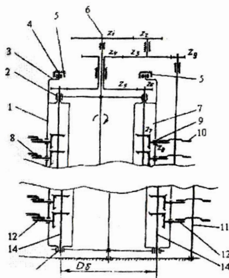
15.4-rasm. Gorizontali shpindelli PTAtining kinematik sxemasi:
