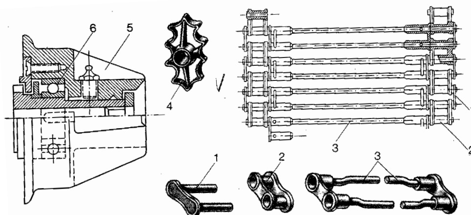
17.4-rasm. Elevatorning qismlari: 1;2–vtulka-rolikli zanjirning qismlari; 3–prutok; 4–tebratish yulduzchasi; 5–rolík; 6–podshipnik
