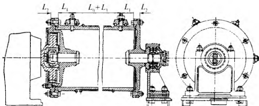
25-rasm. Novsimon ariqchall baraban.
