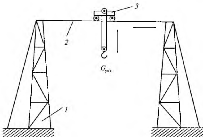
15-rasm. Kabelli kran sxemasi: 1 — ustun tayanch; 2 — arqon; 3 — aravacha.
