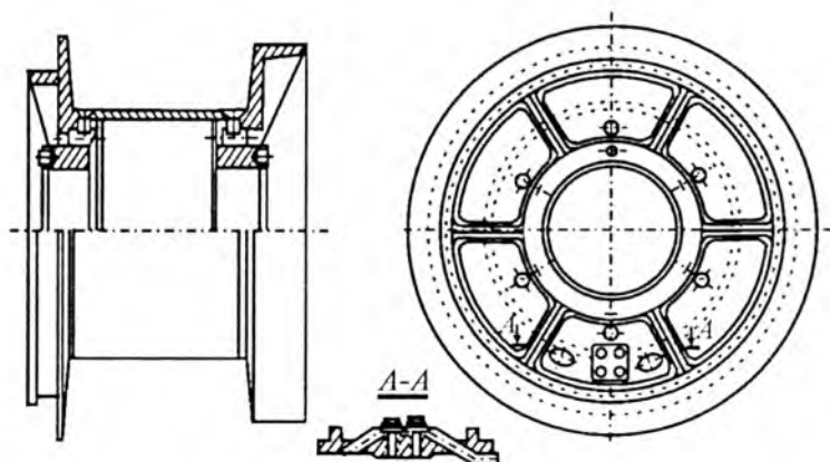
24-rasm. Silliq sirtli baraban.
