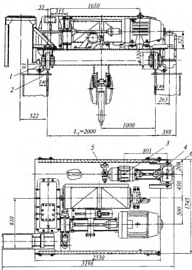
53-rasm. Ko'priqli kran aravachasi:
