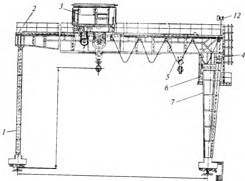
78-rasm. Chorpoyali kran.
