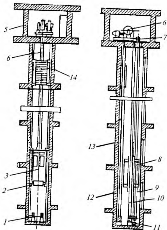
81-rasm. Liftli ko'targich.
