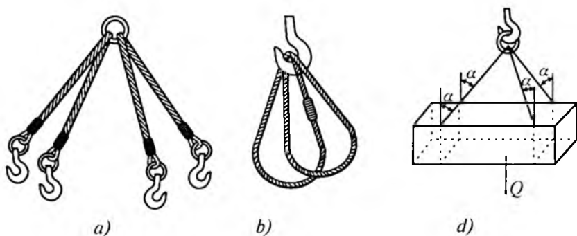
34-rasm. Arqonli stroplar:
