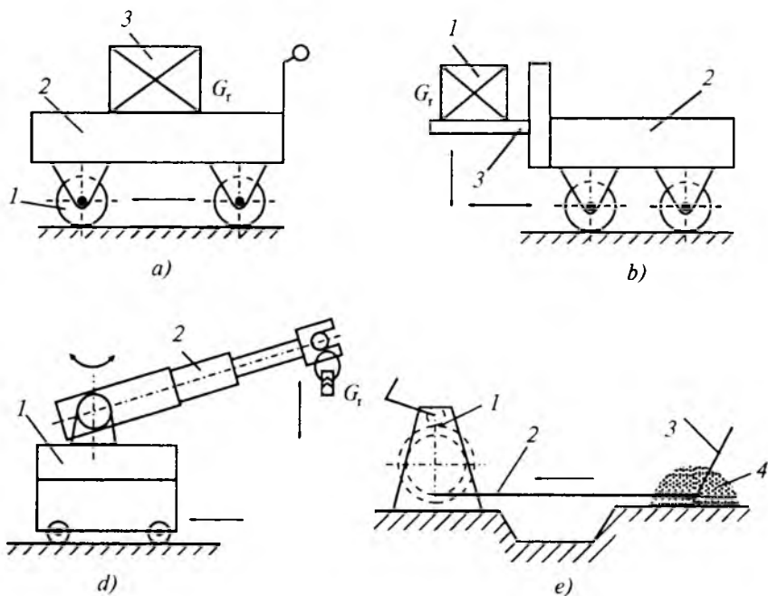
99-rasm. Davriy yuk tashish mashinalarining sxemalari. a — arava; b — elektr yuk ortgich; d — sanoat roboti; e — mexanik belkurak.
