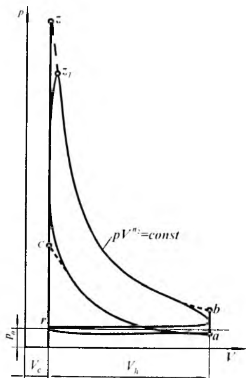
5.11-rasm. Kengayish jarayonining diagrammasi.
