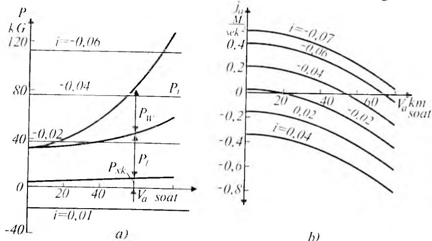
3.9-rasm. Avtomobil g'ildiragiga tortish kuchi ta'sir etmagandagi harakat.
