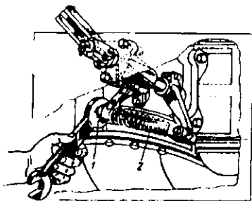
80-rasm. «ZIL-130» avtomobilidagi mexanik yuritmalil ilashma tepkining erkin yo'lini rostdash
