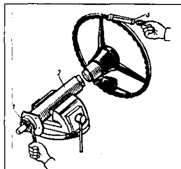
81-rasm. «ZIL-130» avtomobilining rul vali podshipnigini sozlash:
