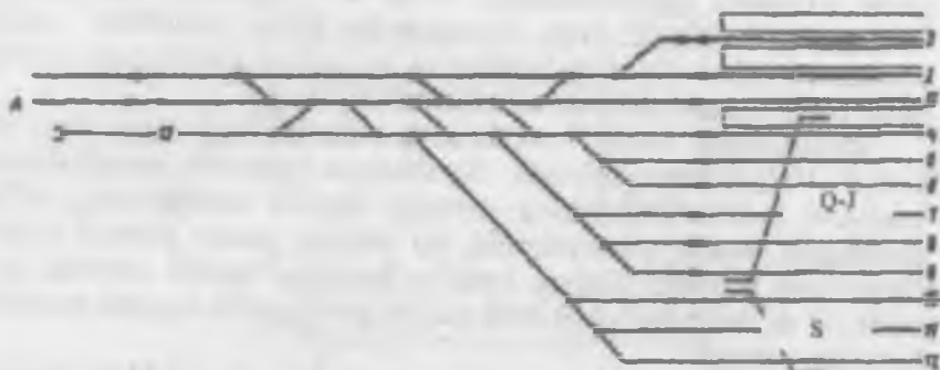
12.1-rasm. Stansiya strelkali bo'g'izining chizmasi: Q - J -qabul-jo'natish parki; S - saralash parki.
