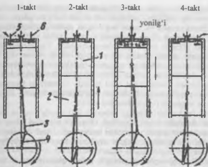
8.10-rasm. To'rt taktli dvigatelning ishlashi: 1-silindr; 2-porshen; 3-shatun; 4-krivoship; 5-purkovchi klapan; 6-chiqaruvchi klapan.
