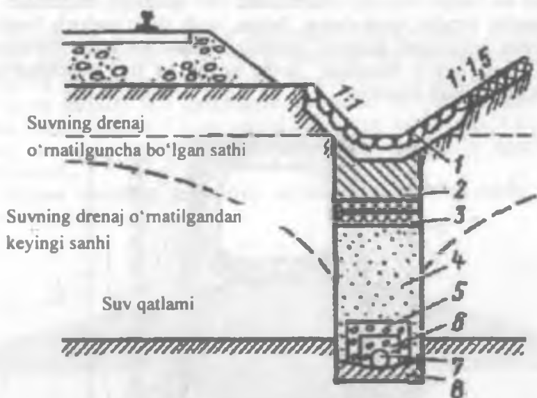
5.6-rasm. Kyuvetosti drenaj: 1 — mustahkamlangan qatlam; 2 — shibbalangan qatlam; 3 — ikki o'ovak qatlam; 4 — yirik qum; 5 — shcheben yoki mayda tosh; 6 — shcheben yoki yirik tosh; 7 — drenaj quvuri; 8 — yassi yog'och.
