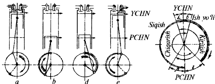
4.2-rasm. Gaz taqsimlash diagrammasi:
