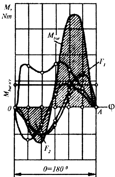
14.8-rasm. To'rt silindrli, to'rt taktli motorning yig'indi burovchi moment grafigini chizish
