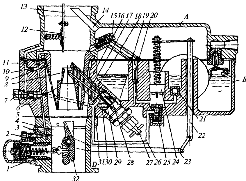
6.10-rasm. Diffuzordagi siyraklanishni o'zgartirib dozalovchi karburator (K-22T) ning sxemasi:
