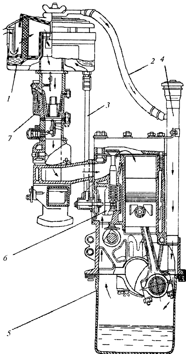
9.8-rasm. Motor karterini shamollatish sxemasi: 1 — havo tozalagich; 2 va 3 — quvurcha; 4 — moy quyish quvuri; 5 — karter; 6 — klapanlar qutisi; 7 — karburator
