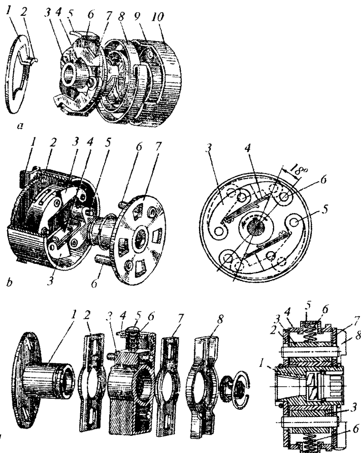
11.4-rasm. Yurgizish tezlatgichi (a) va yondirishni ilgarilash muftalari (b, d):
