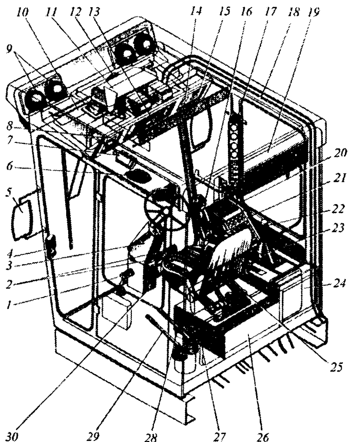
28.3- rasm. Haydovchi kabinasining ishchi o'rne:
