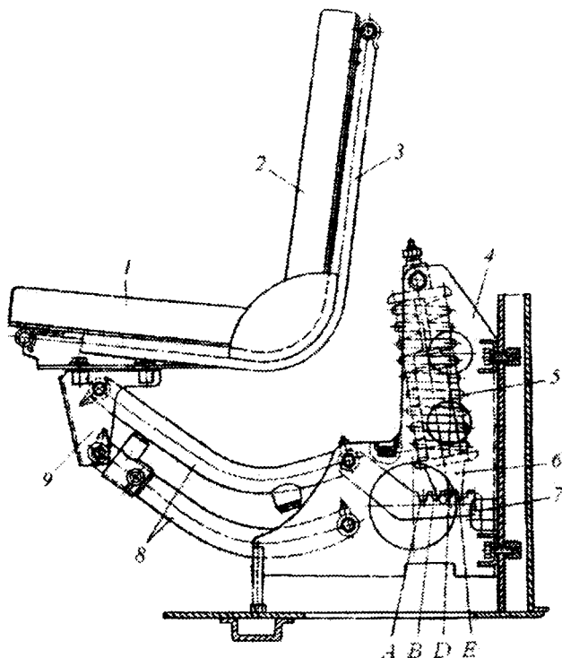
28.5-rasm. Traktorchining resorlangan o'rindig'i:
