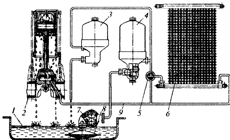
9.1-rasm. Motor moylash tizimining sxemasi:
