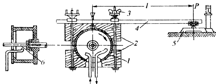
13.1-rasm. Mexanik tormozning sxemasi: 1 — shkv; 2 — kolodka; 3 — quloqli gayka; 4 — richag; 5 — tarozi; 6 — sterjen
