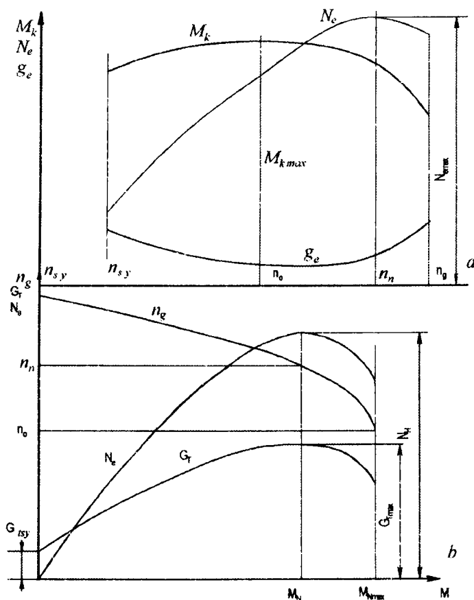
22.3-rasm. Motorning regulator tavsiflari:
