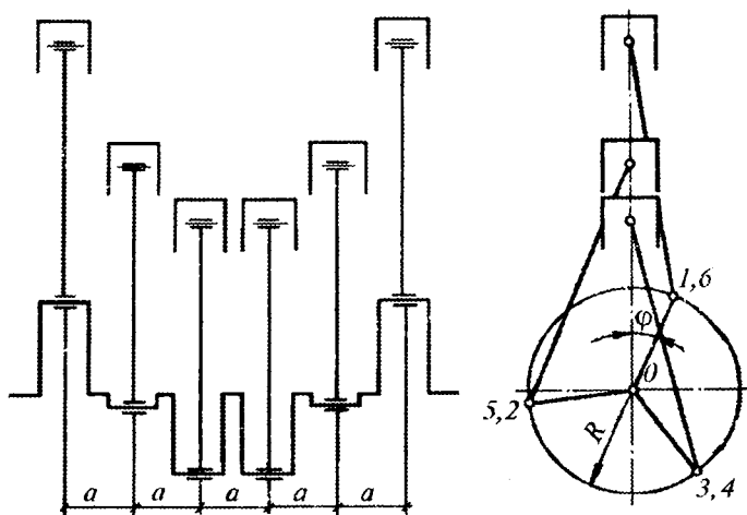
14.11-rasm. Olti silindrlı, to'rt taktli motorni muvozanatlash
