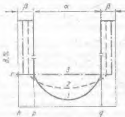
2.4-rasm. v –fazaning chegarasida boshlang'ich (1), oraliq (2) va yakunlovchi (3) gomogenlash momentida b –eritmaning dendritli yacheykasining kesimida legirolovchi elementlarning taqsimlanishining egri chizig'i.
