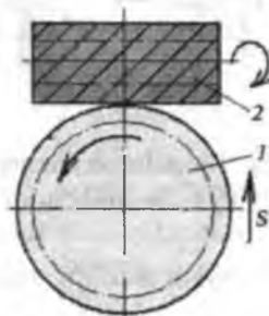
5.25-rasm. Chervyakli g'ildirakni radial surish bilan kesish:
