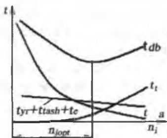
8.3-rasm. Sozlashda: t_{db} — donabay vaqtga keskich asboblarning sonining ta'siri.
