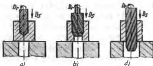
5.9 -rasm. Teshiklarga ishlov berish usullari: a—parmalash; b—zekerlash; d—razvyorkalash.
