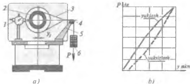
2.19-rasm. K.V. Votinovning tokarlik dastgohi bikrligini statik aniqlash:
