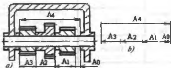
11.2-rasm. Yig'ish o'lchamlar zanjiri sxemasi:
