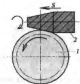
5.26-rasm. Chervyakli g'ildirakni tangensial surish bilan kesish:
