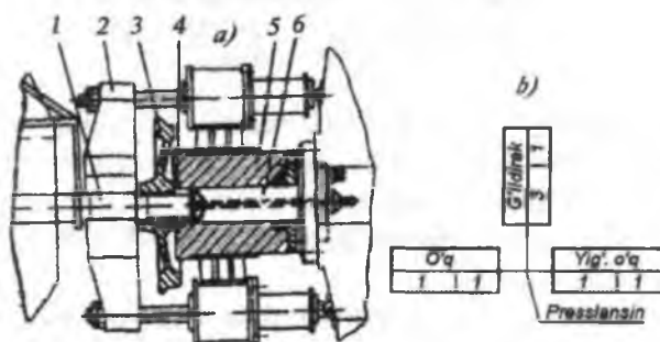
12.4-rasm. G'ildirak juftligini gidroresslab yig'ish:
