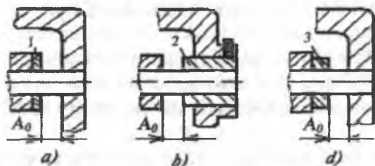
11.1-rasm. Yig'ish sxemalari:
