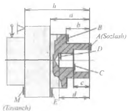
3.17-rasm. Tanavorni tokarlik-revolver dastgohida ishlov berishda sozlash bazasini qo'llash misoli.
