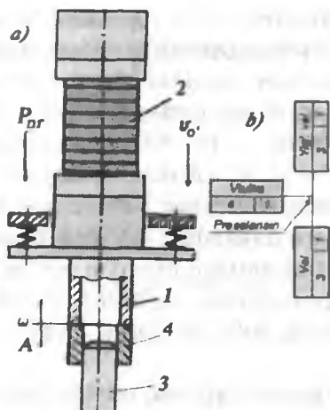
12.3-rasm. Ultratovushli presslash:
