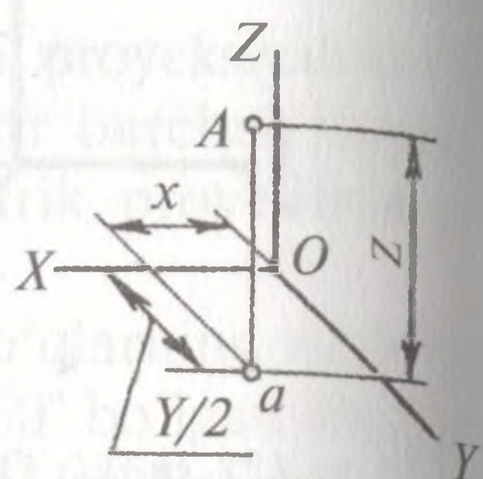
Qiyshiq burchakli (frontal) diametriya
