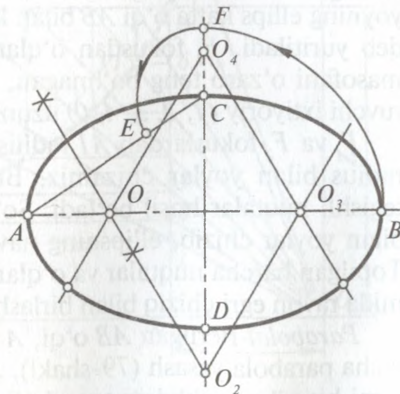
77-shakl. To'rt markazli oval yasash.
