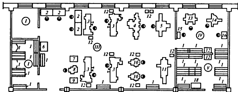
7.13 - rasm. Asbobsozlik bo'limining ko'rinishi:
