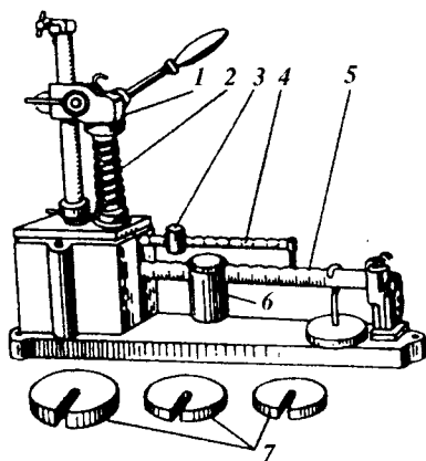
4.29 - rasm. Prujinalarning bikirligini nazorat qilish moslamasi:
