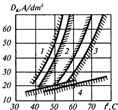
5.12-rasm. Xromlash tartibining xromli qatlam turiga ta'siri:
