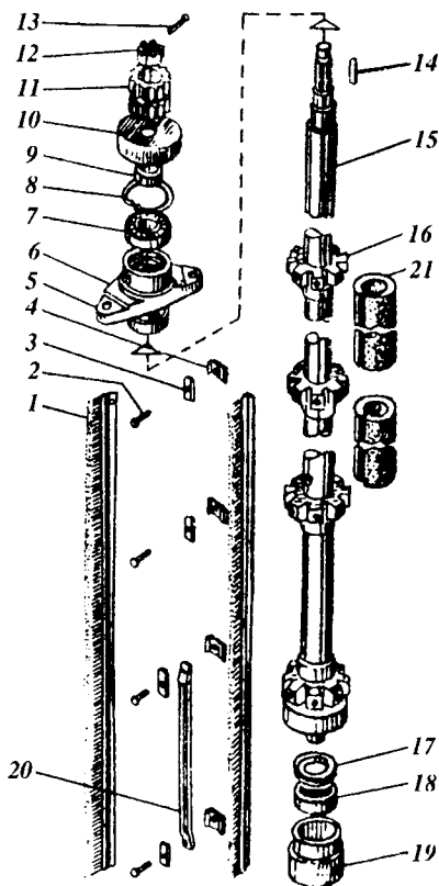
4.16 - rasm. Cho'tkali ajratkich: 1 — cho'tka plankalari; 2 — bolt; 3 — shayba; 4 — qulf; 5, 17 — manjeta; 6 — yuqorigi qopqoq; 7, 18 — podshipnik; 8 — mahkamlash halqasi; 9 — vtulka; 10 — qopqoq; 11 — shesternya; 12 — gayka; 13 — shplint; 14 — shponka; 15 — val; 16 — separator; 19 — pastki qopqoq; 20 — planka; 21 — egiluvchan vtulka.
