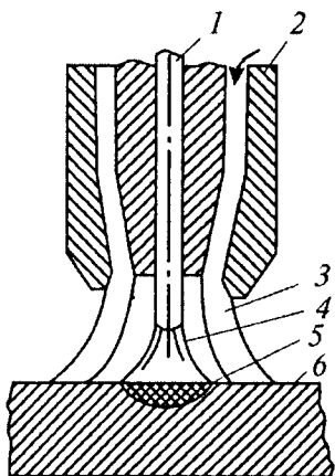
5.4-rasm. Karbonat angidrid gazi muhitida payvandlash sxemasi:
