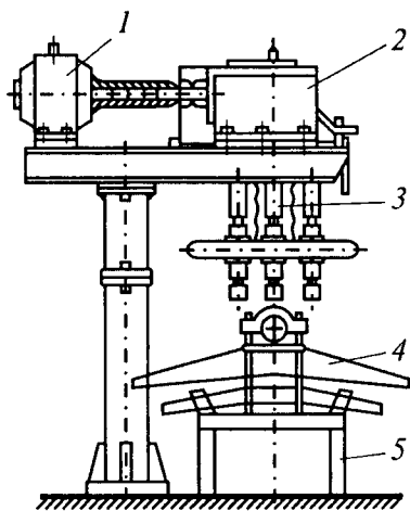
4.13 - rasm. Ressor tirgovuchlarining gaykalarini burab chiqarish stendi: 1 — elektr dvigatel; 2 — reduktor; 3 — shpindel; 4 — ressor; 5 — taglik.
