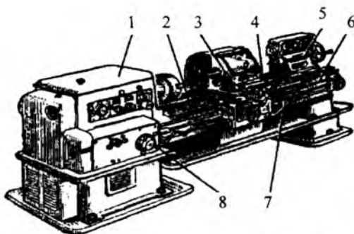
10.5-rasm. 1K62 markali tokartik-vint qirqish dastgohi:
