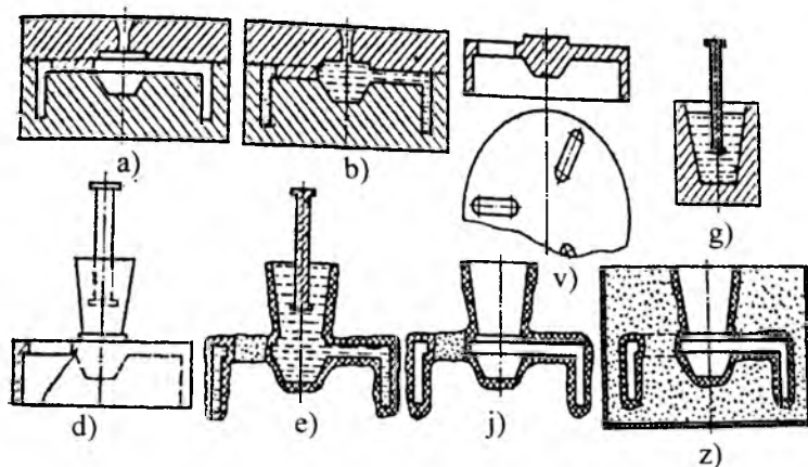
7.32-rasm. Eritiladigan modellarda quyma olish sxemasi: a) press-forma; b) model qorishmasili press forma; v) model, g) modelning quyish tizimini tayyorlash, d) model bloki; e) qobig'li model bloki; j) qobig'li shakl; z) shakllangan qobig'.
