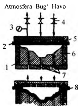
11.11-rasm. Listdan vakuumdan yoki havo (yohud bug') bosimidan foydalanib, matritsaga yo'nalgan botirish usulida shtamplash.
