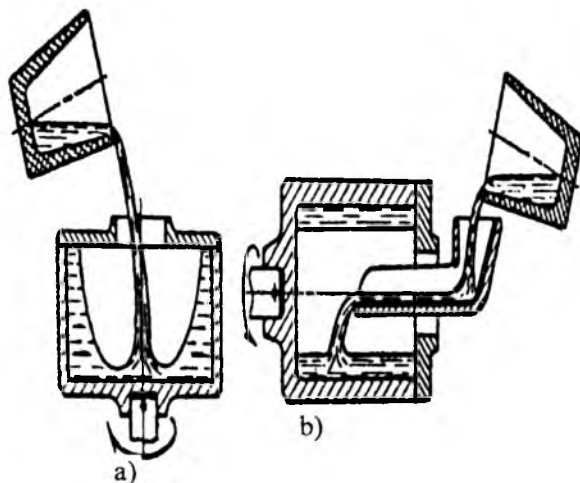
7.25-rasm. Markazdan qochirma kuch usulida quyma quyish sxemasi: a) vertikal o'q aylanishi bo'ylab quyish; b) gorizontal o'q aylanishi bo'ylab quyish.
