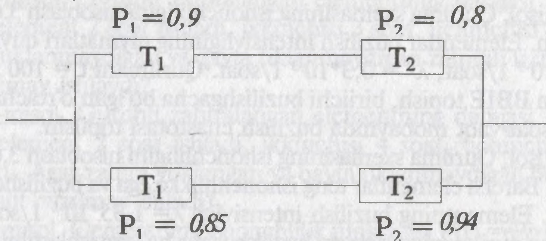
3.3-rasm. Sxema ishonchliligini hisoblash.
