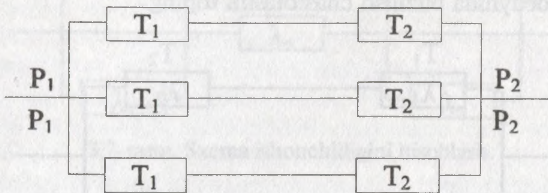
3.2-rasm. Ishonchlilik sxemasini hisoblash.
