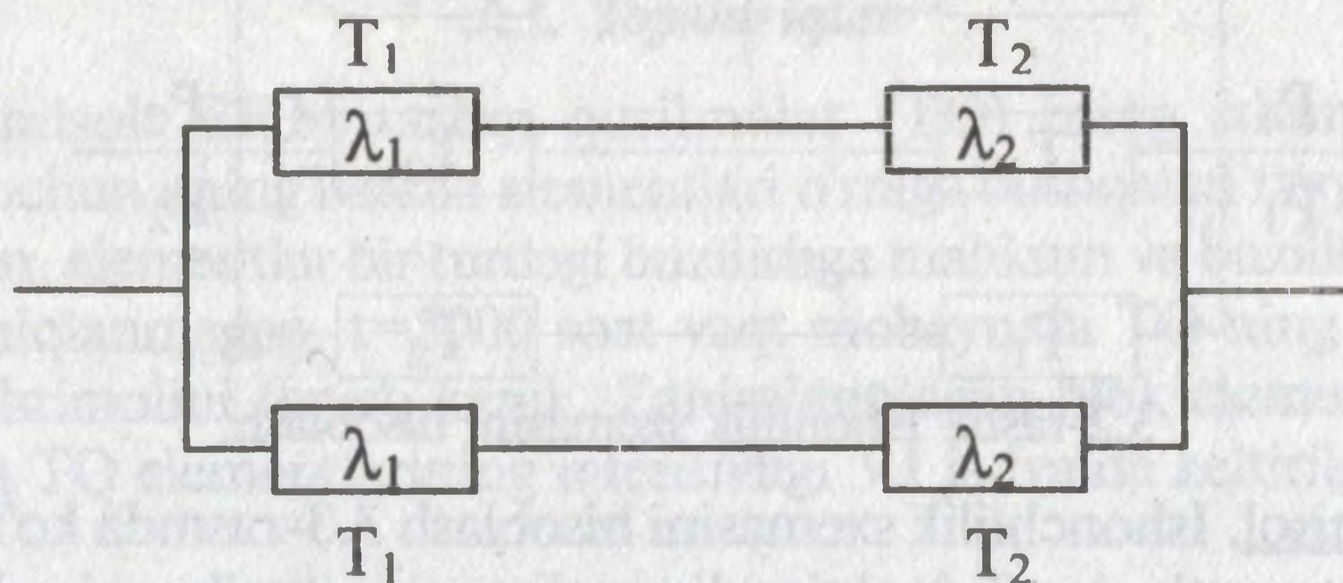
3.5. rasm. Sxema ishonchliligini hisoblash.
