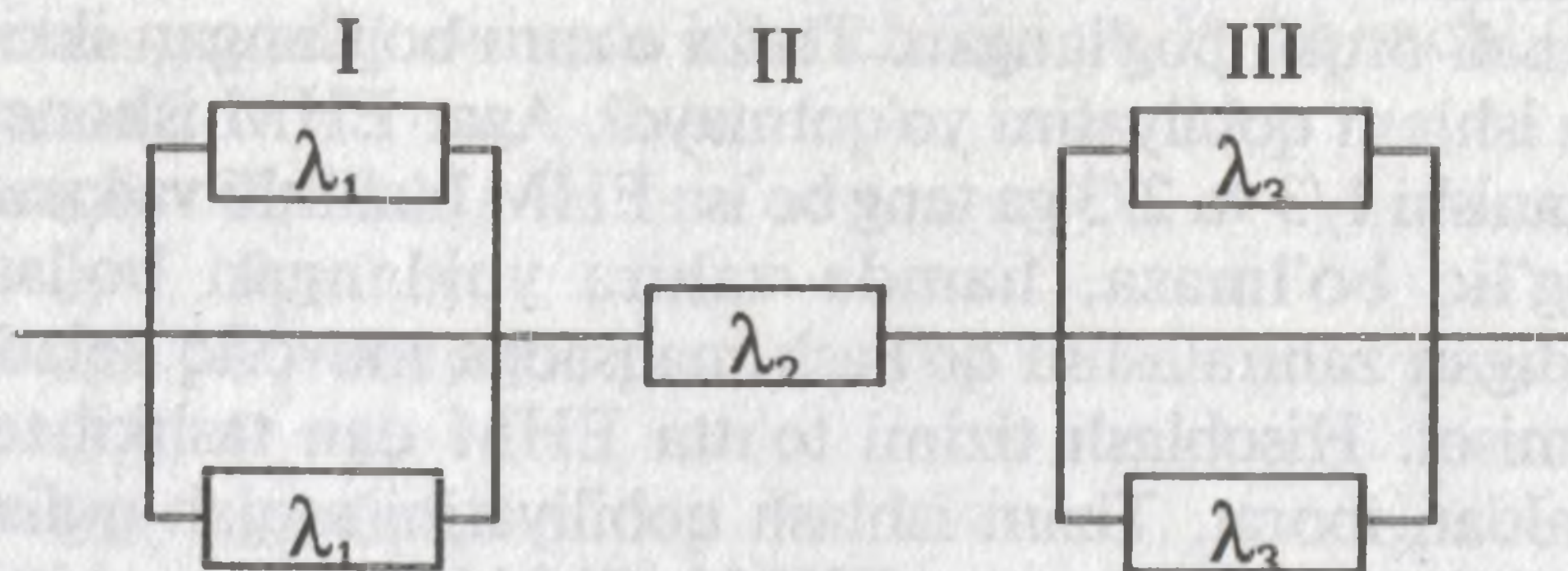
3.7-rasm. Sxema ishonchliligini hisoblash.
