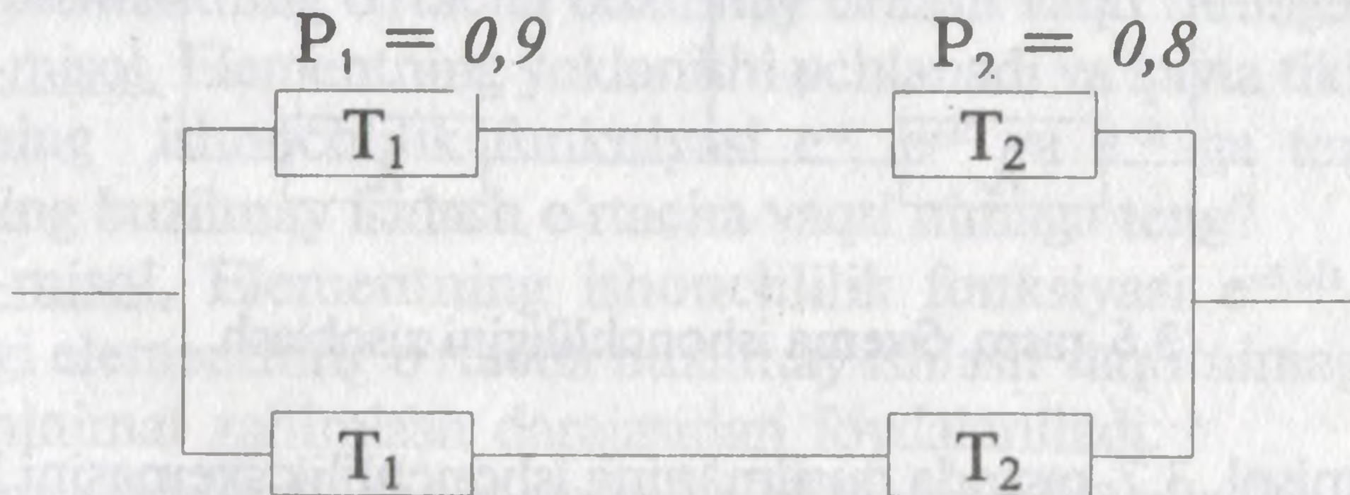
3.4-rasm. Sxema ishonchliligini hisoblash.
