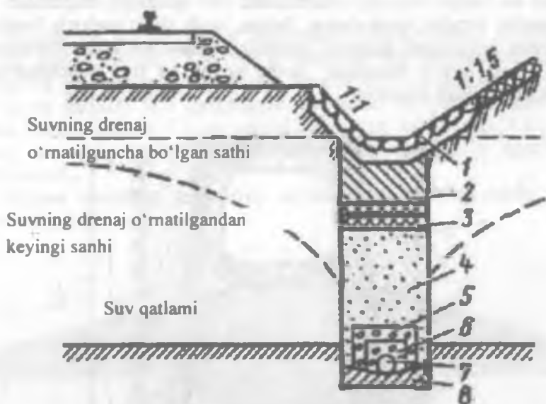
5.6-rasm. Kyuvetosti drenaj: 1 — mustahkamlangan qatlam; 2 — shibbalangan qatlam; 3 — ikki o'vak qatlam; 4 — yirik qum; 5 — shcheben yoki mayda tosh; 6 — shcheben yoki yirik tosh; 7 — drenaj quvuri; 8 — yassi yog'och.
