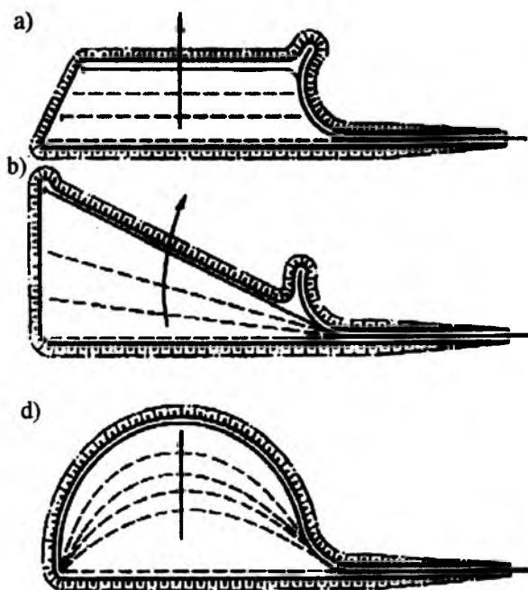
45-rasm. Ag'darma ish frontining surulish usullari:
