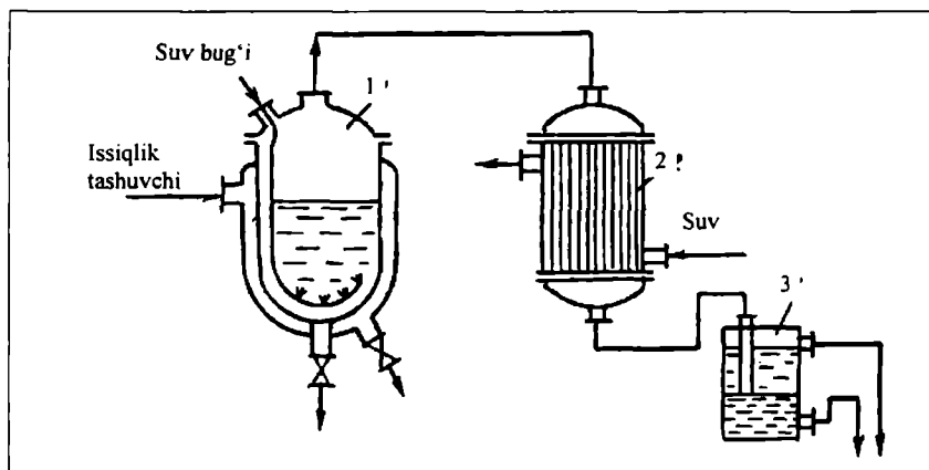
13.4-rasm. Suv bug'i bilan haydash qurilmasining sxemasi: 1–bug' g'illofli haydash kubi; 2–kondensator-sovitgich; 3–separator.
