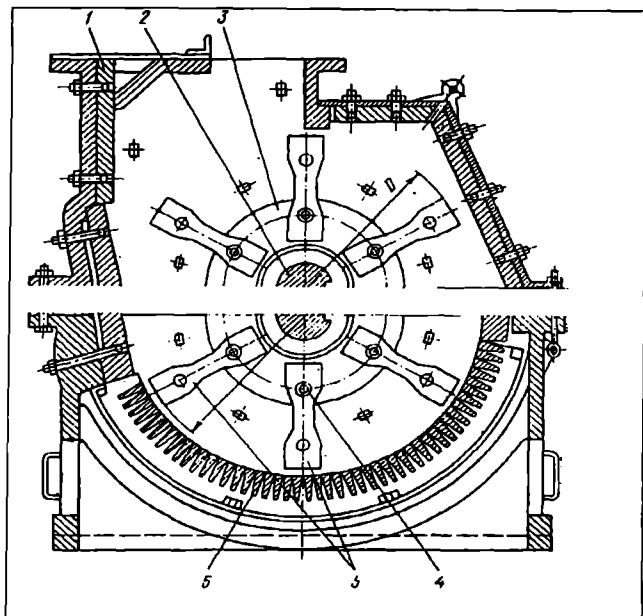
7.3-rasm. Bol'g'ali yanchish mashinasi: 1-qobiq; 2-val; 3-disk; 4-paleslar; 5-bolg'achalar; 6-kolosnikli panjara.
