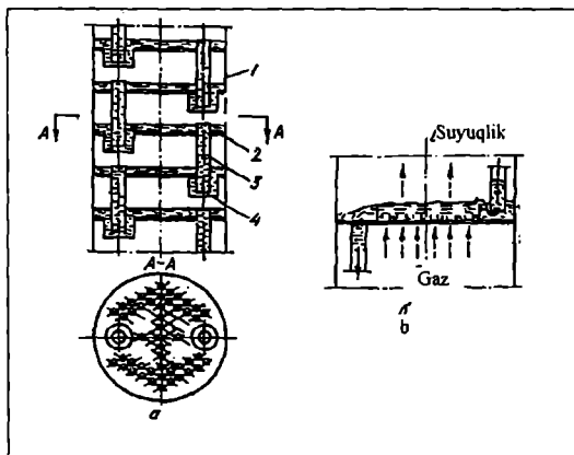
15.4-rasm. Elaksimontarelkali kolonna: a–kolonnaning tuzilishi; b–tarelkaning ishlash prinsipi; 1–qobiq; 2–tarelka; 3–quyilish quvuri, 4–stakan.
