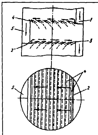
15.6-rasm. Plastinali tarelka:
