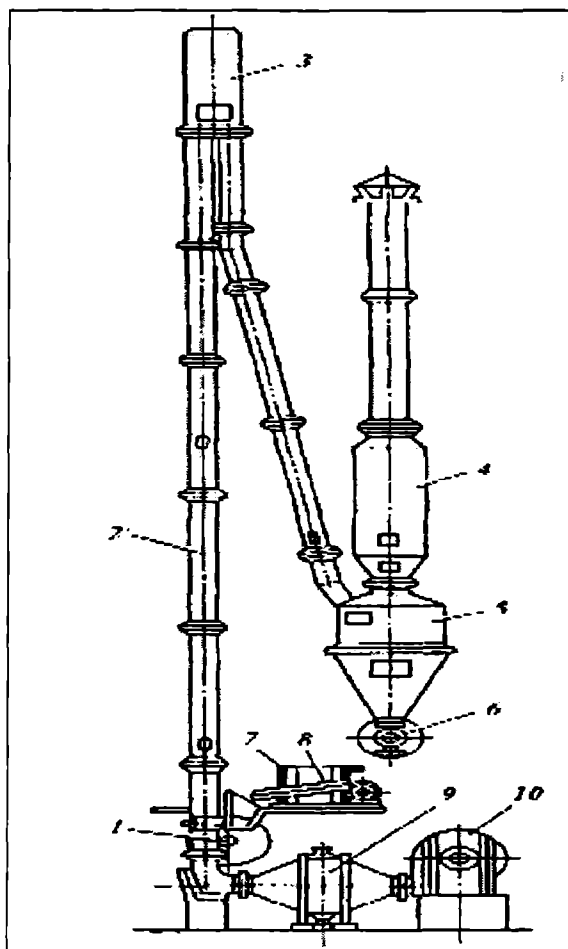
18.12-rasm. Pnevmatik quritgich:
