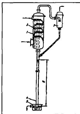
10.17-rasm. Qarama-qarshi yo‘nalishli barometrik kondensator: 1—kondensator; 2—tomchi ushlagich; 3—tokchalar; 4—barometrik quvur; 5—barometrik idish.
