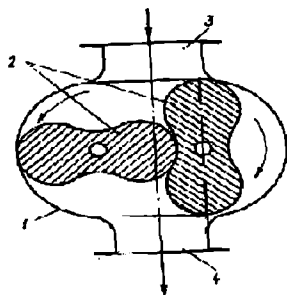
3.29- rasm. Rotatsion gazoduvka:
