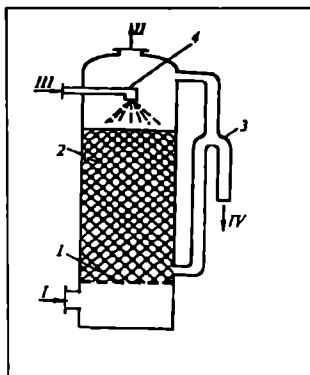
15.14-rasm. Nasadkali emulgatsion kolonna:
