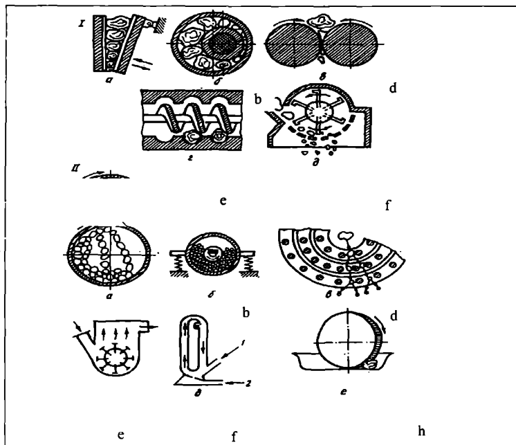
7.2-rasm. Maydalash mashinalarining prinsipial sxemalari:
