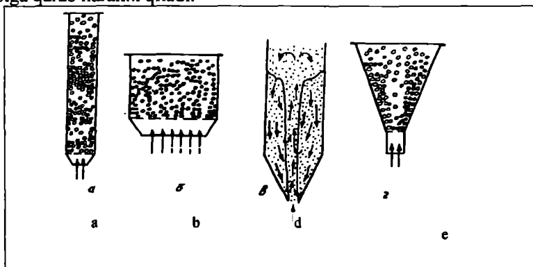
6.2-rasm. Mavhum qaynash qatlamining turlari:
