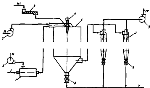
18.13-rasm. Mahsulot sohib beriladigan quritgich:
