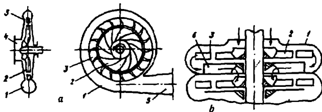
3.22- rasm. Turbogazoduvkalar:
