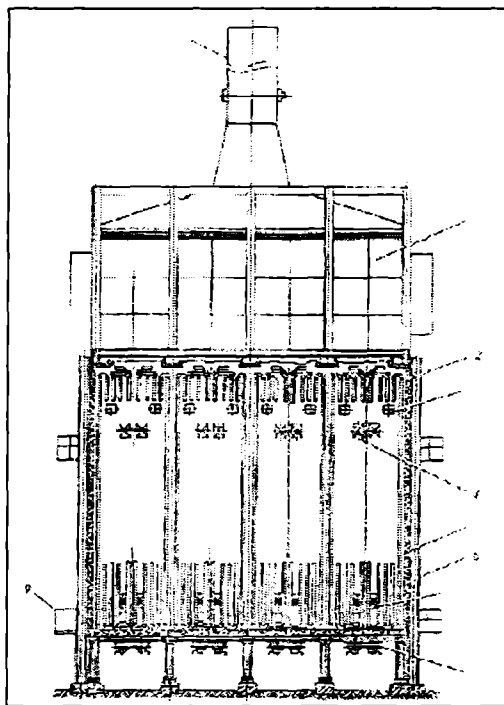
11.4-rasm. VS rusumidagi quvurli pech sxemasi:
