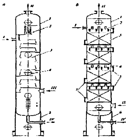
14.7-rasm. Absorberlar:
