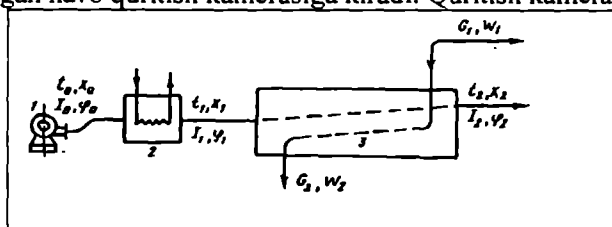
18.6-rasm. Normal quritish jarayonining sxemasi: 1—ventilator; 2—kalorifer; 3—quritish kamerasi.
