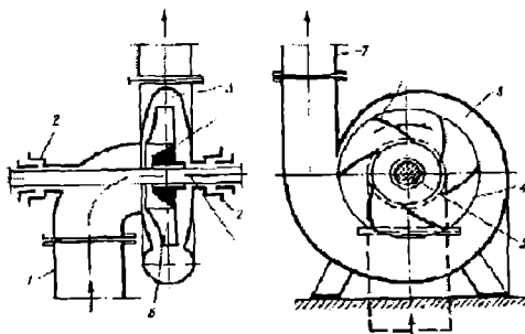
3.2-rasm. Markazdan qochma nasos:
