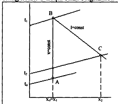
18.7-rasm. Nazariy quritish jarayonining I - x diagrammasida tasvirlash.
