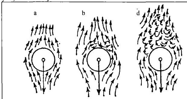
4.2-rasm. Qattiq sharsimon zarrachning suyuqlikdagi harakati: a – laminar oqim; b – oraliq oqim; d – turbulent oqim.
