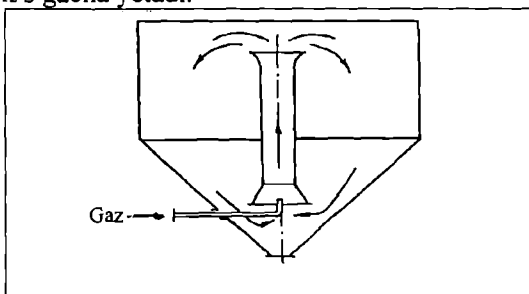
5.4-rasm. Erliftdan foydalanilgan aralashtirgich.
