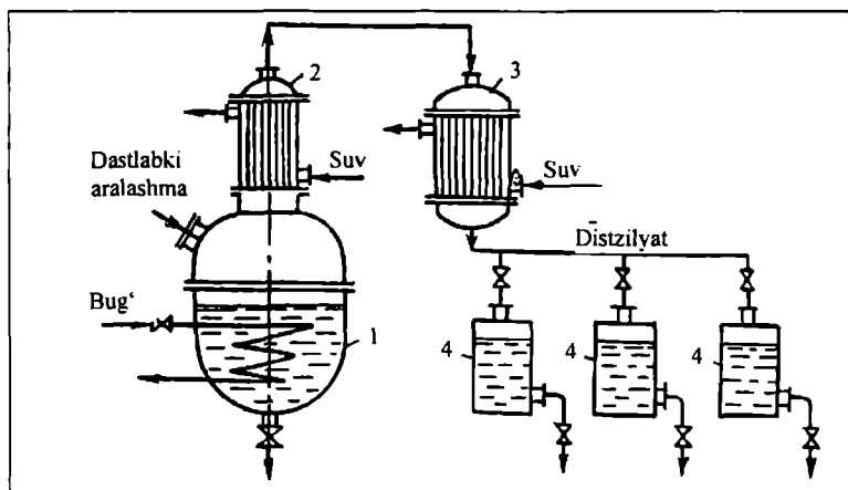
13.3-rasm. Deflegmatsiyali oddiy haydash qurilmasining sxemasi: 1–haydash kubi; 2–deflegmator; 3–kondensator-sovitkich; 4–yig'gich.
