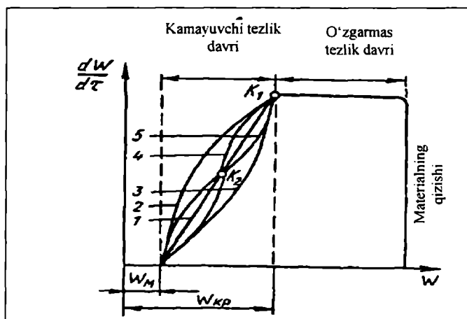
18.5-rasm. Quritish tezligining egri chizig'i:
