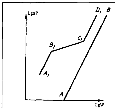
15.3-rasm. Tarelkali absorberlarning gidrodinamik rejimlari: AB—quruq tarelkaning ishlash rejimi; A_1V_1 —pufakli rejim; V_1S_1 —ko'pikli rejim; C_1D_1 —ingichka oqimli(injeksion) rejim.
