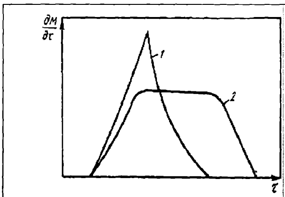
19.2-rasm. Kristallanish tezligining vaqtdan bog‘liqligi: 1–eritmaning to‘yinish darajasi nisbatan katta bo‘lganda; 2–o‘ta to‘yinish darajasi kichik bo‘lganda.
