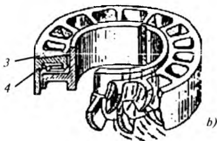
4.15-rasm. Turbobur.
