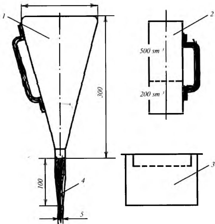
7.3- rasm. CIB-5 standart dala viskozimetri: 1 – voronka; 2 – o'lchov idishi; 3 – to'r; 4 – trubka
