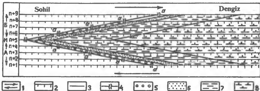
72-rasm. Uchinchi fatsial zonallik qonunini tushuntiruvchi chizma.
