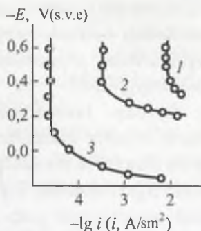
4.21-rasm. Erish tezligining potensialga bog'lanishi:
