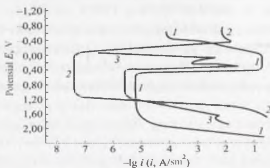
7.2-rasm. Turli metallar uchun erish tezligining potentsialga bog'liqligi
