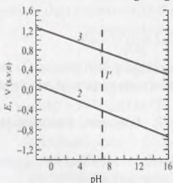
4.2-rasm. 25°S haroratda suv uchun E—pH diagrammasi
