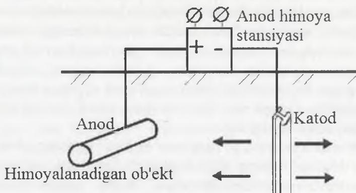
10.4-rasm. Anodli himoyalash sxemasi
