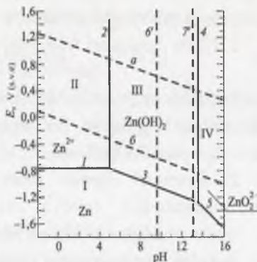
4.3-rasm. Zn—H 2 O sistemasi uchun E—pH diagrammasi.
