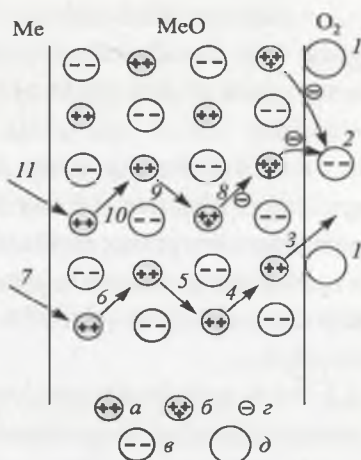
3.14-rasm. \text{Cu}_2\text{O} turdagi plyonkaning o'sishidagi diffuziya sxemasi.
