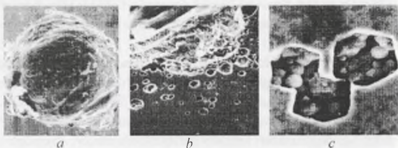
5.1-rasm. 03X18N11markali zanglamaydigan po'lat sirtidagi yirik pitting.
