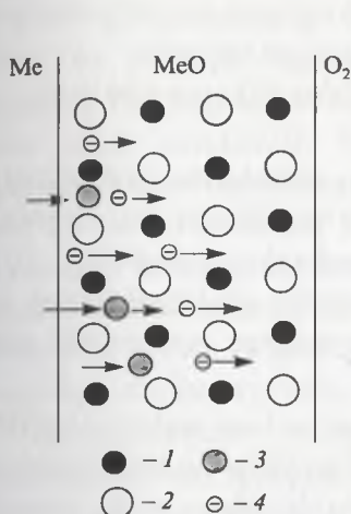
3.13-rasm. \text{ZnO} turdagi plyonkaning o'sishidagi diffuziya sxemasi.
