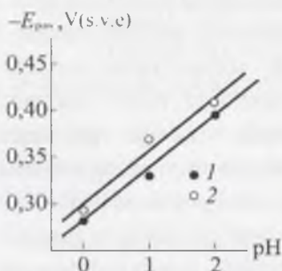
4.23-rasm. Xrom passivlanish potentsia-lining ( E_{pas} ) muhit pH ga bog'liqligi.
