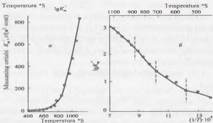
3.17-rasm. Temir oksidlanishining K_m^+ — harorat (a) va \lg K_m^+ — 1/T (b) koordinatalaridagi haroratga bog'liqligi
