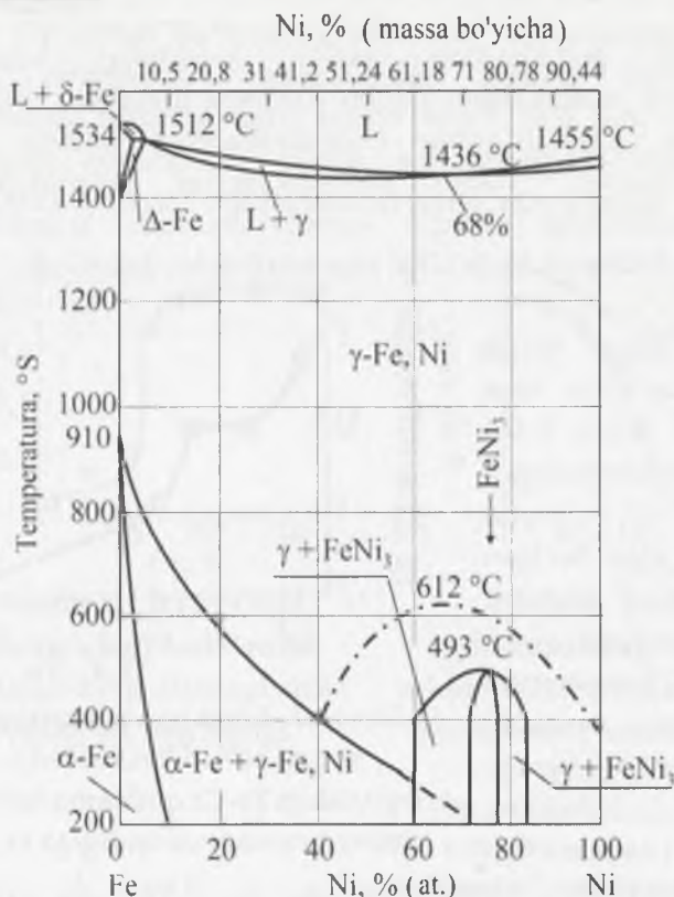
7.7-rasm. Fe-Ni sistemasining holat diagrammasi
