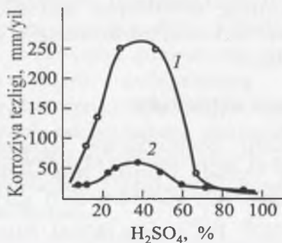
10.7-rasm. Po'lat korroziyalanish tezligining \text{H}_2\text{SO}_4
