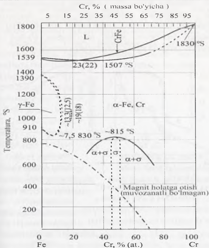
7.3-rasm. Fe-Cr sistemasining holat diagrammasi
