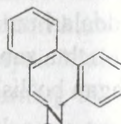
fenantridin
