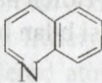
xinolin
