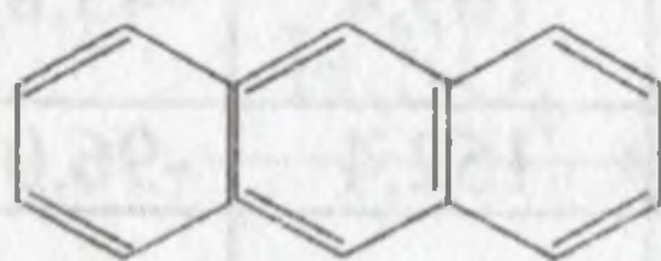
antrotsen
