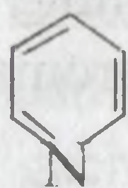
piridin
