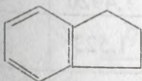
Indan
