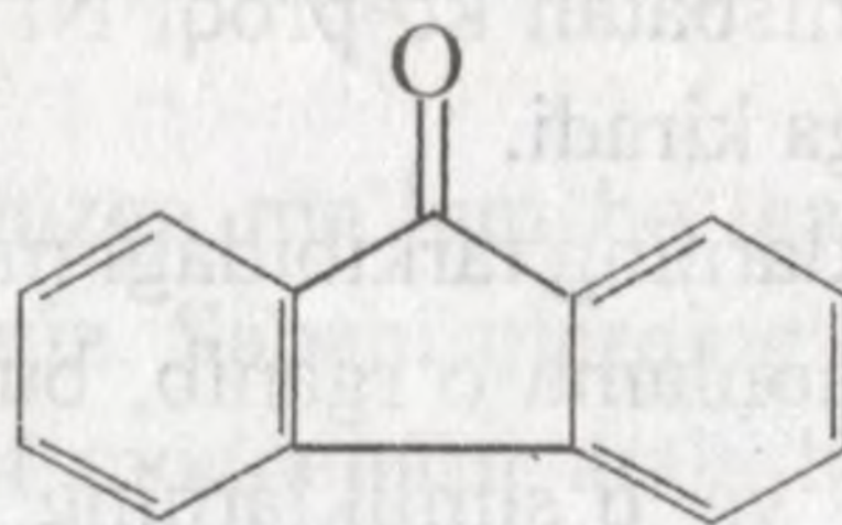
fluorenon
