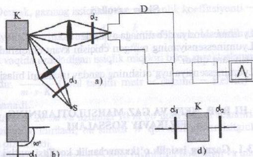
2.10-rasm. Lyuminessent qurilmani yig'ish usullari.
